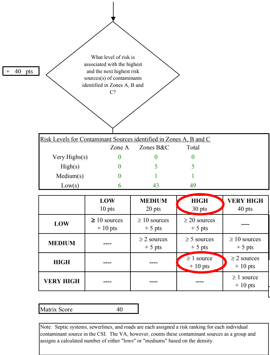
Chart 9. Contaminant risks for KPBSD Kalifornsky Beach Elementary - Heavy Metals, Cyanide and Other Inorganic Chemicals
