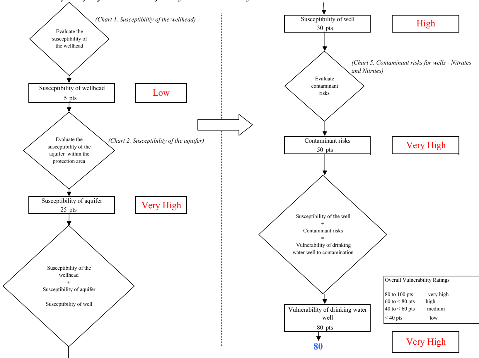
Chart 6. Vulnerability analysis for KPBSD Kalifornsky Beach Elementary - Nitrates and Nitrites
