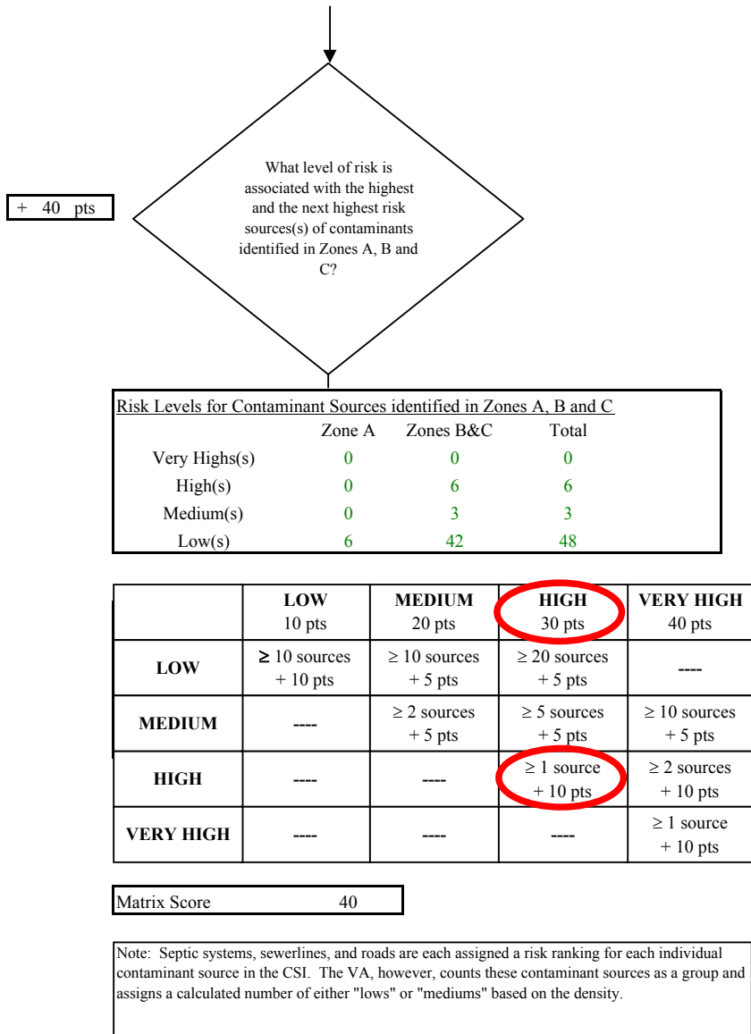
Chart 7. Contaminant risks for KPBSD Kalifornsky Beach Elementary - Volatile Organic Chemicals
