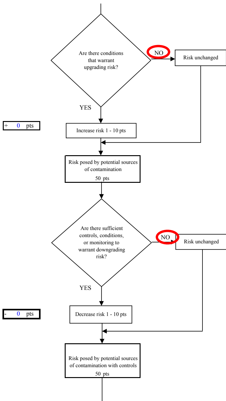
Chart 5. Contaminant risks for KPBSD Kalifornsky Beach Elementary - Nitrates and Nitrites
