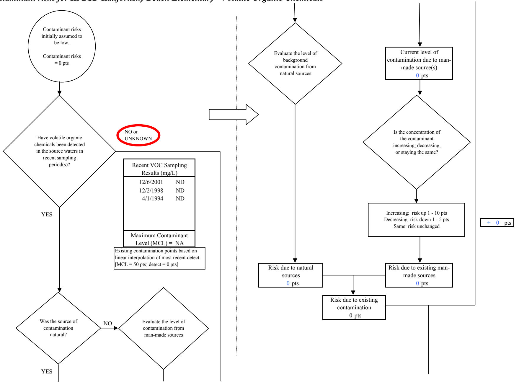
Chart 7. Contaminant risks for KPBSD Kalifornsky Beach Elementary - Volatile Organic Chemicals
