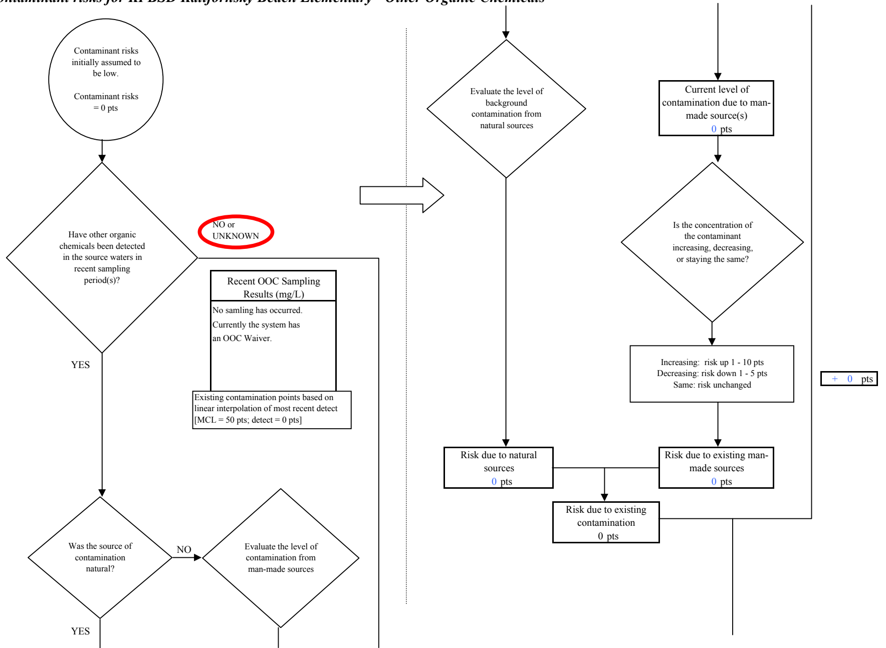
Chart 13. Contaminant risks for KPBSD Kalifornsky Beach Elementary - Other Organic Chemicals
