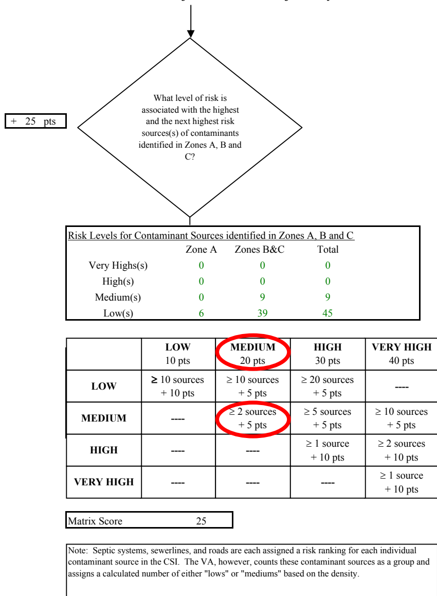
Chart 13. Contaminant risks for KPBSD Kalifornsky Beach Elementary - Other Organic Chemicals
