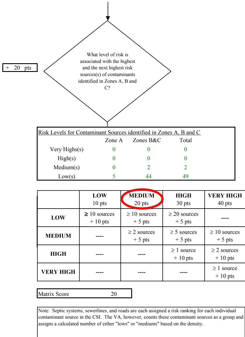
Chart 11. Contaminant risks for KPBSD Kalifornsky Beach Elementary - Synthetic Organic Chemicals
