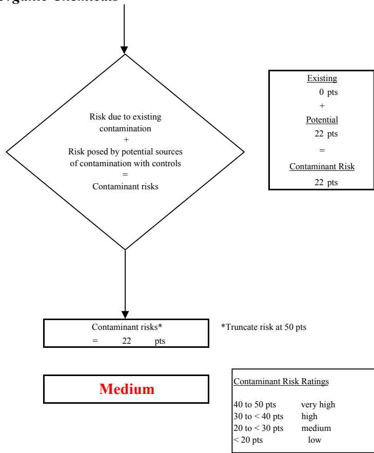
Chart 11. Contaminant risks for KPBSD Kalifornsky Beach Elementary - Synthetic Organic Chemicals
