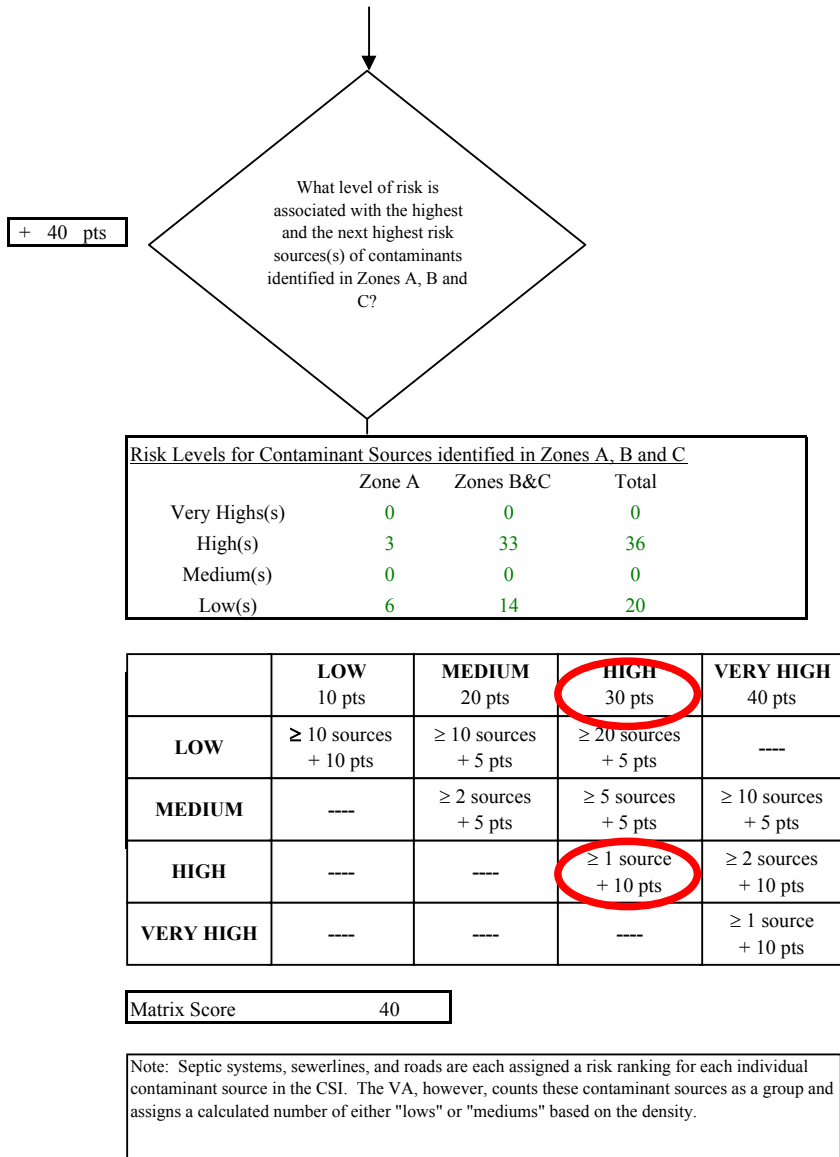
Chart 5. Contaminant risks for KPBSD Kalifornsky Beach Elementary - Nitrates and Nitrites
