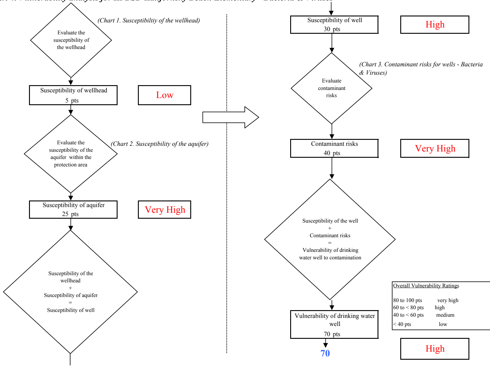
Chart 4. Vulnerability analysis for KPBSD Kalifornsky Beach Elementary - Bacteria & Viruses
