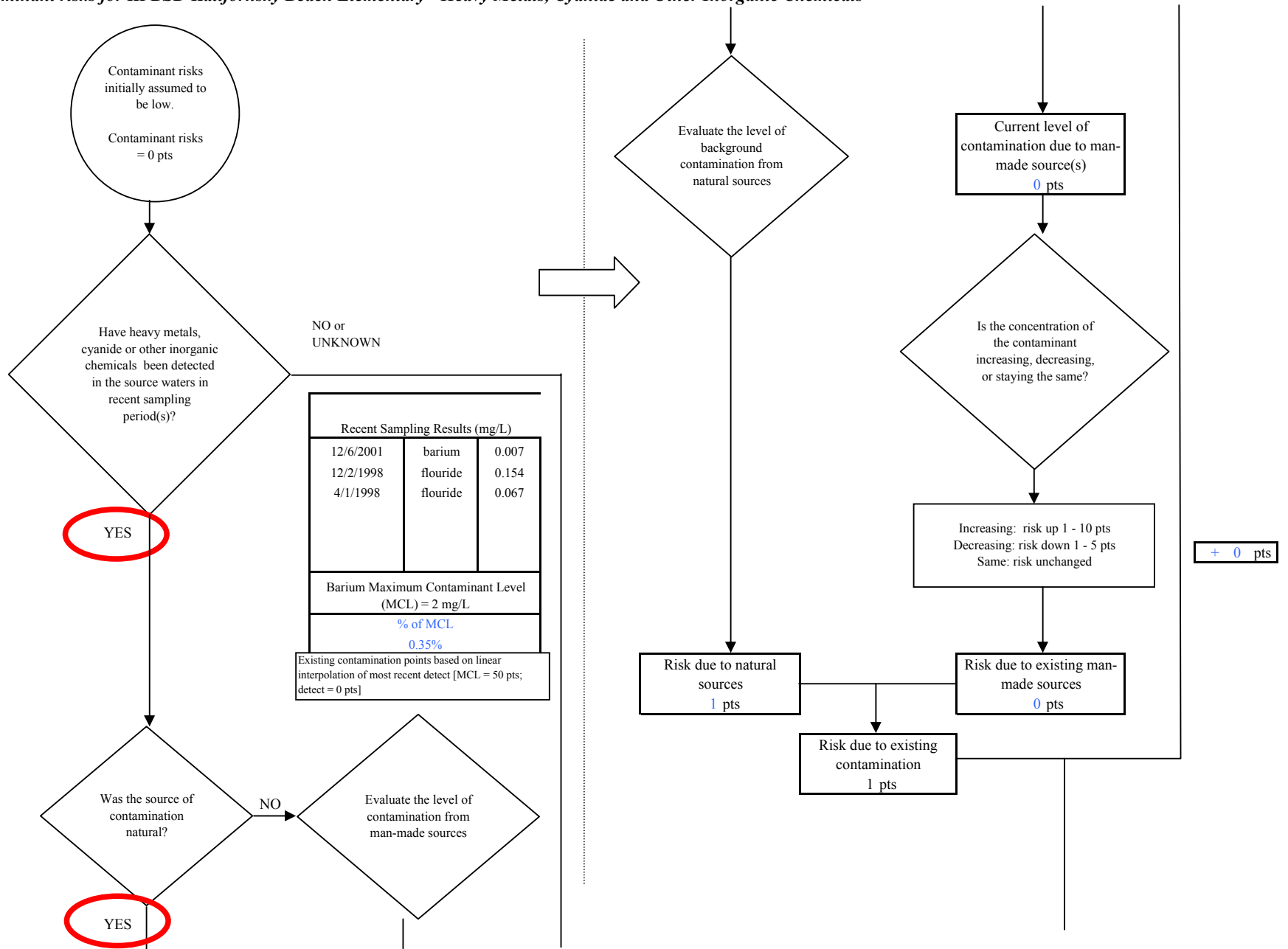
Chart 9. Contaminant risks for KPBSD Kalifornsky Beach Elementary - Heavy Metals, Cyanide and Other Inorganic Chemicals
