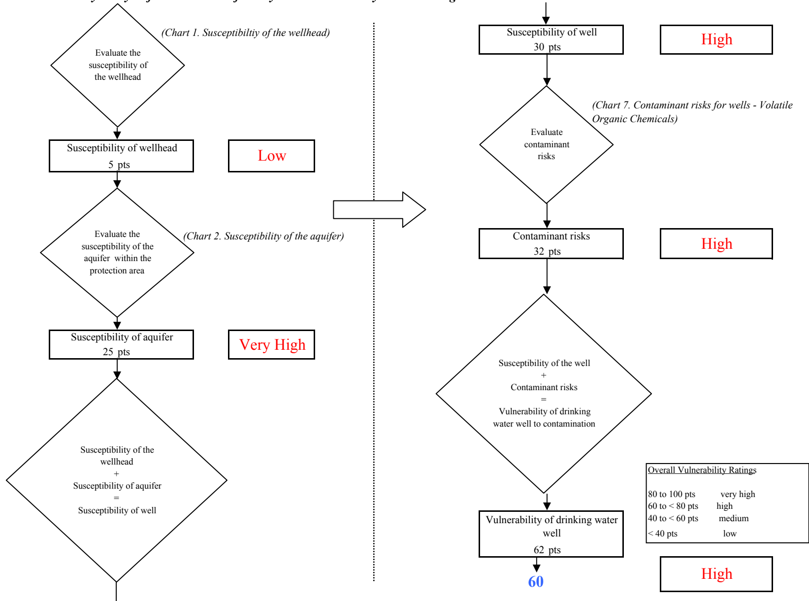
Chart 8. Vulnerability analysis for KPBSD Kalifornsky Beach Elementary - Volatile Organic Chemicals
