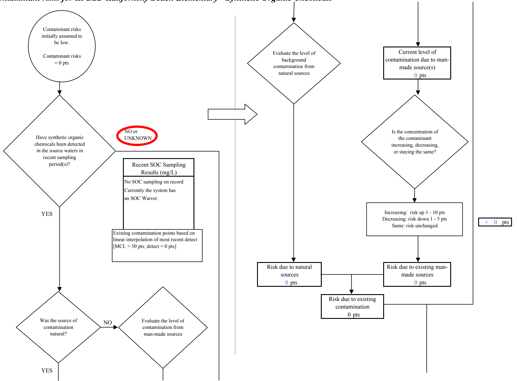
Chart 11. Contaminant risks for KPBSD Kalifornsky Beach Elementary - Synthetic Organic Chemicals
