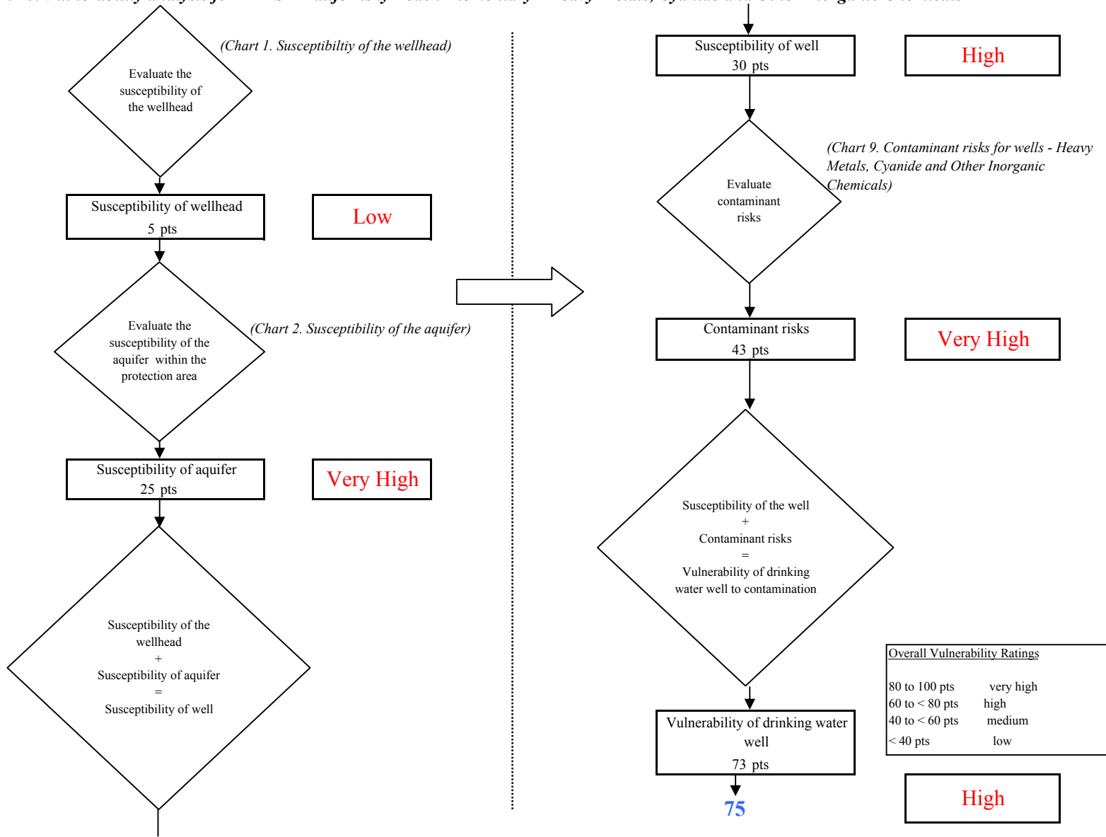
Chart 10. Vulnerability analysis for KPBSD Kalifornsky Beach Elementary - Heavy Metals, Cyanide and Other Inorganic Chemicals
