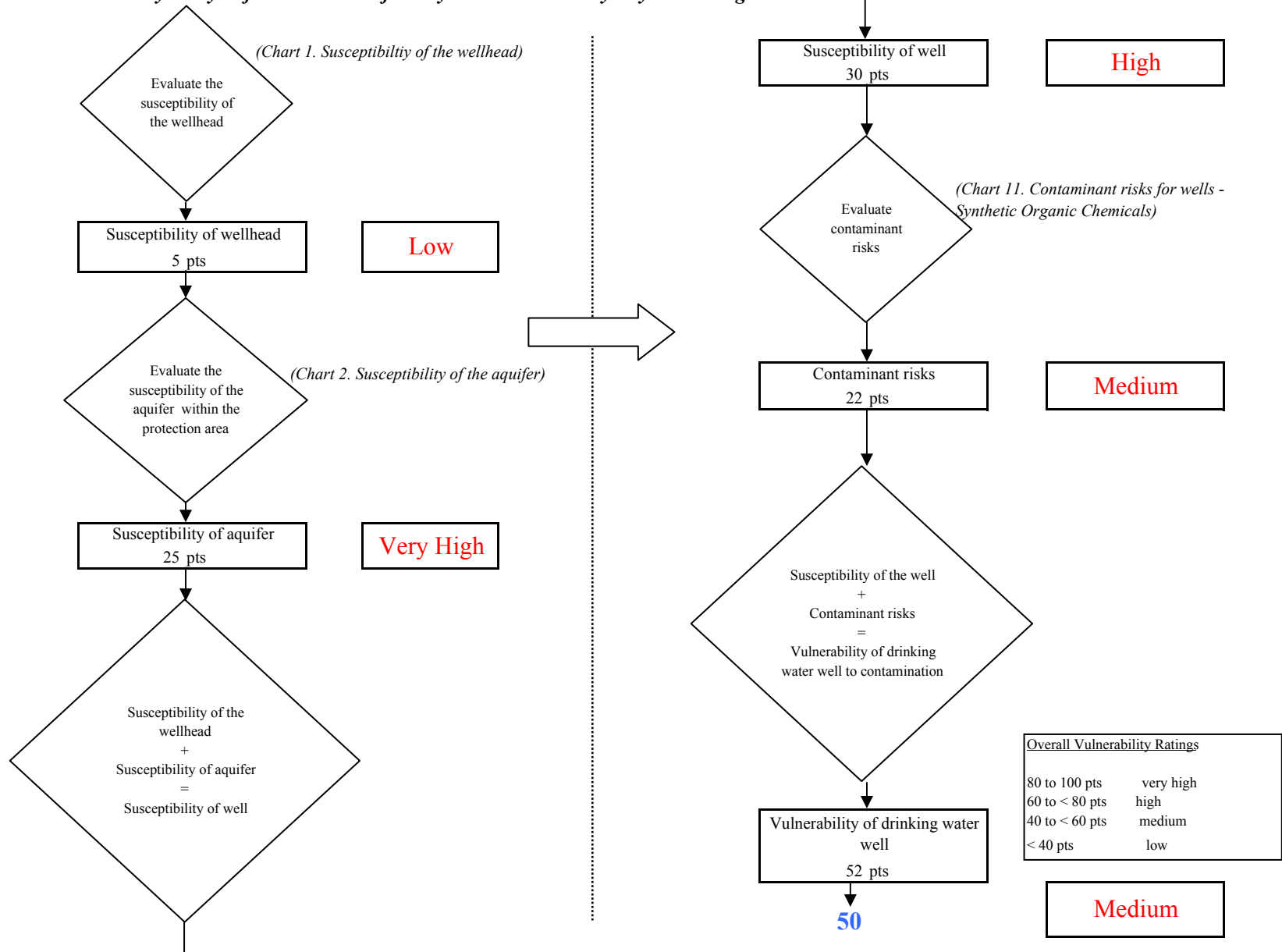
Chart 12. Vulnerability analysis for KPBSD Kalifornsky Beach Elementary - Synthetic Organic Chemicals
