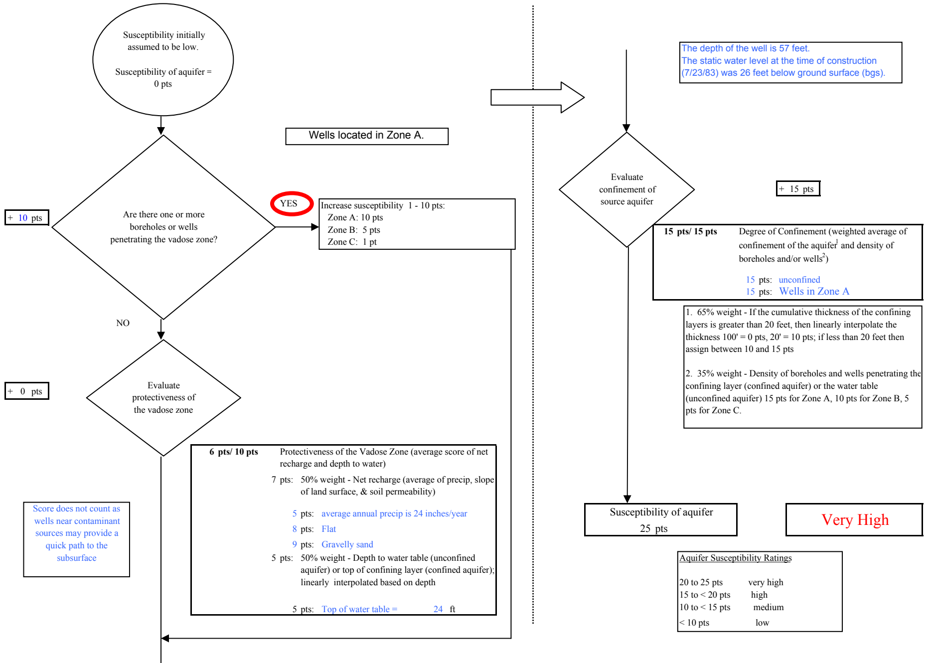
Chart 2. Susceptibility of the aquifer - KPBSD Kalifornsky Beach Elementary
