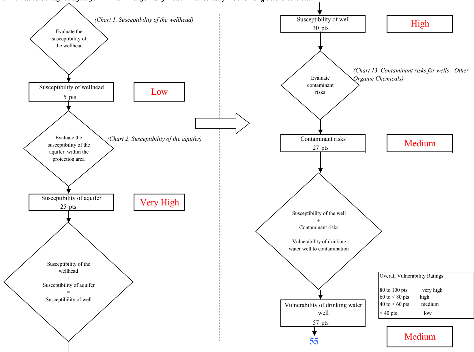
Chart 14. Vulnerability analysis for KPBSD Kalifornsky Beach Elementary - Other Organic Chemicals
