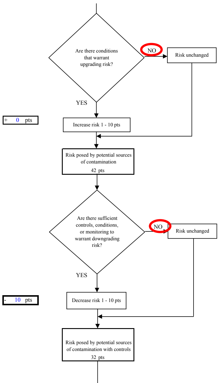
Chart 7. Contaminant risks for KPBSD Kalifornsky Beach Elementary - Volatile Organic Chemicals
