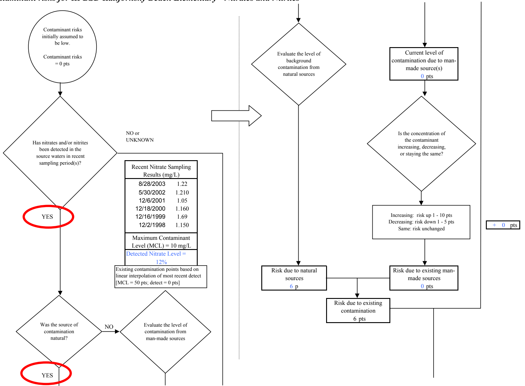
Chart 5. Contaminant risks for KPBSD Kalifornsky Beach Elementary - Nitrates and Nitrites
