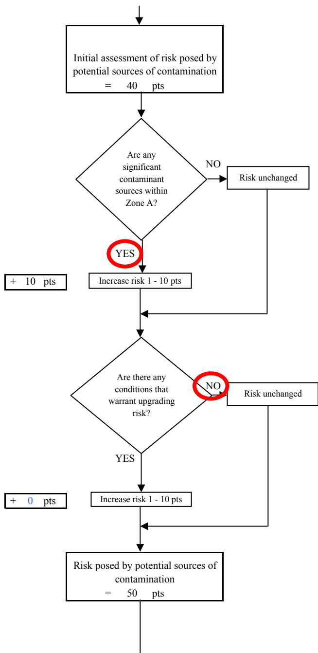
Chart 3. Contaminant risks for KPBSD Kalifornsky Beach Elementary - Bacteria & Viruses
