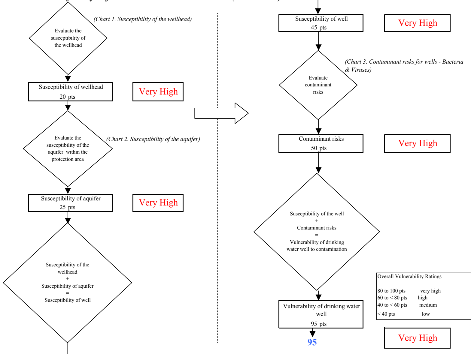
Chart 4. Vulnerability analysis for Inlet Fish Producers - Kenai (241444.002) - Bacteria & Viruses
