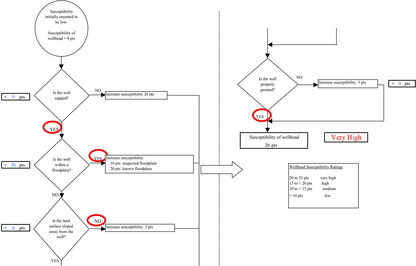
Chart 1. Susceptibility of the wellhead - Inlet Fish Producers - Kenai (241444.002)
