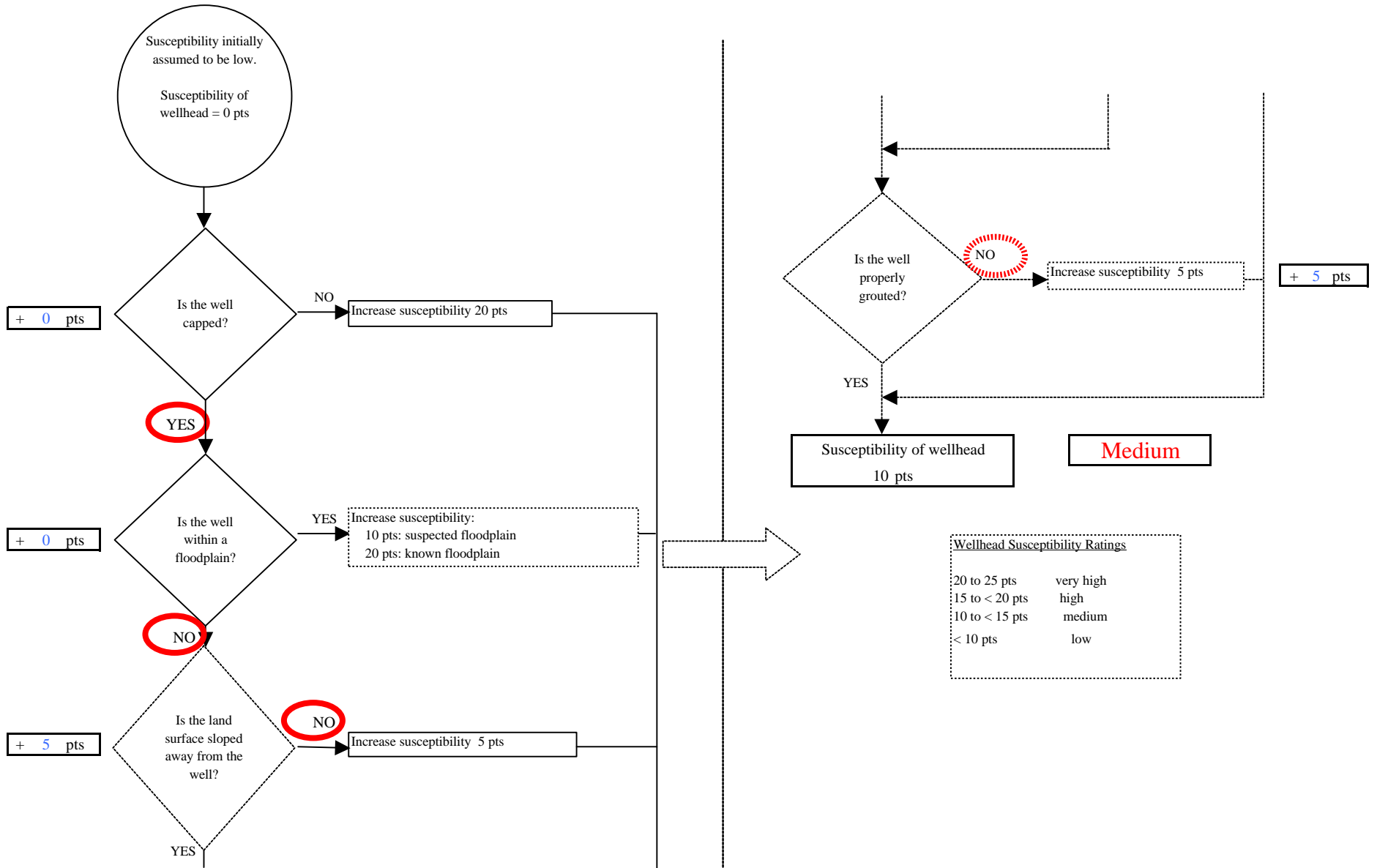
Chart 1. Susceptibility of the wellhead - Totem Inn
