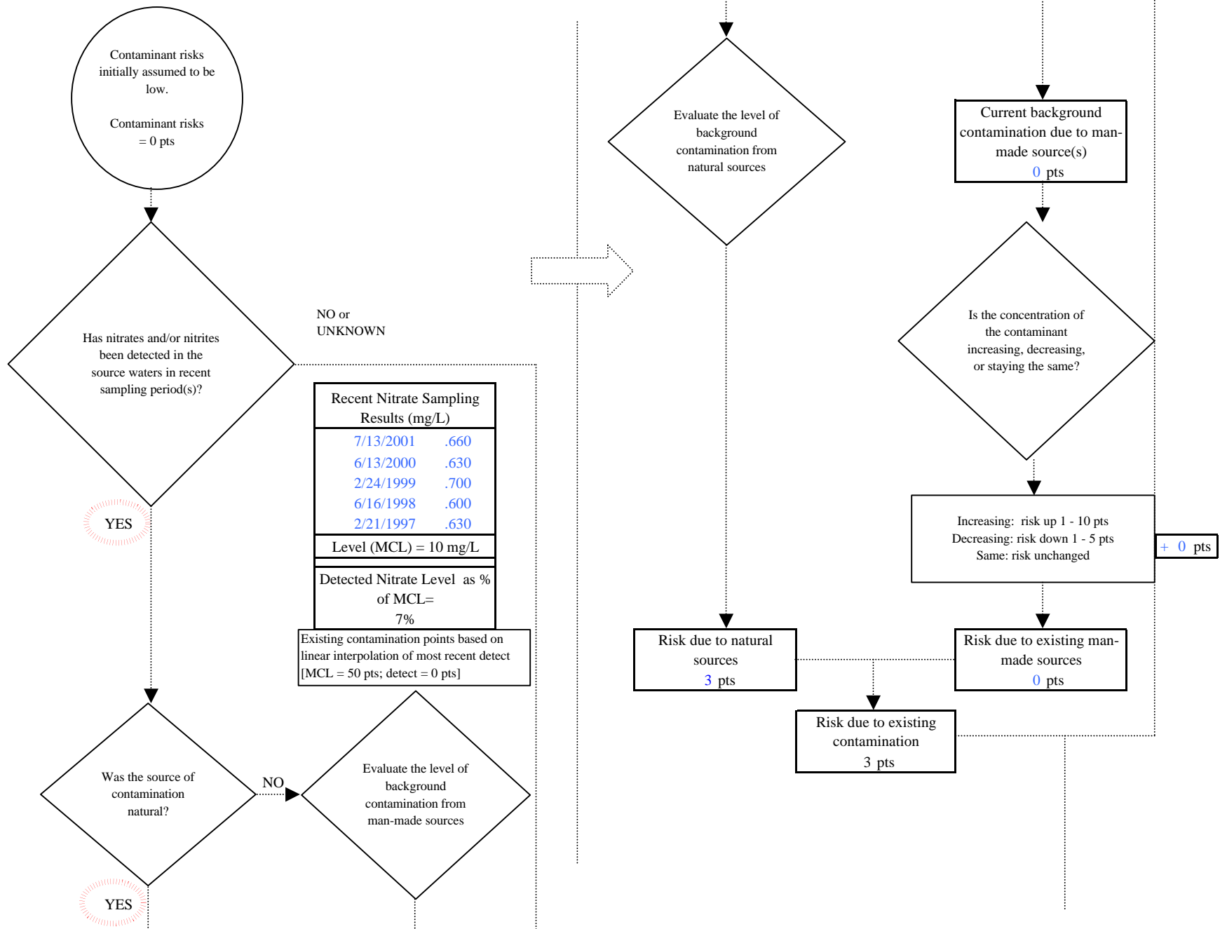
Chart 5. Contaminant risks for Totem Inn - Nitrates and Nitrites
