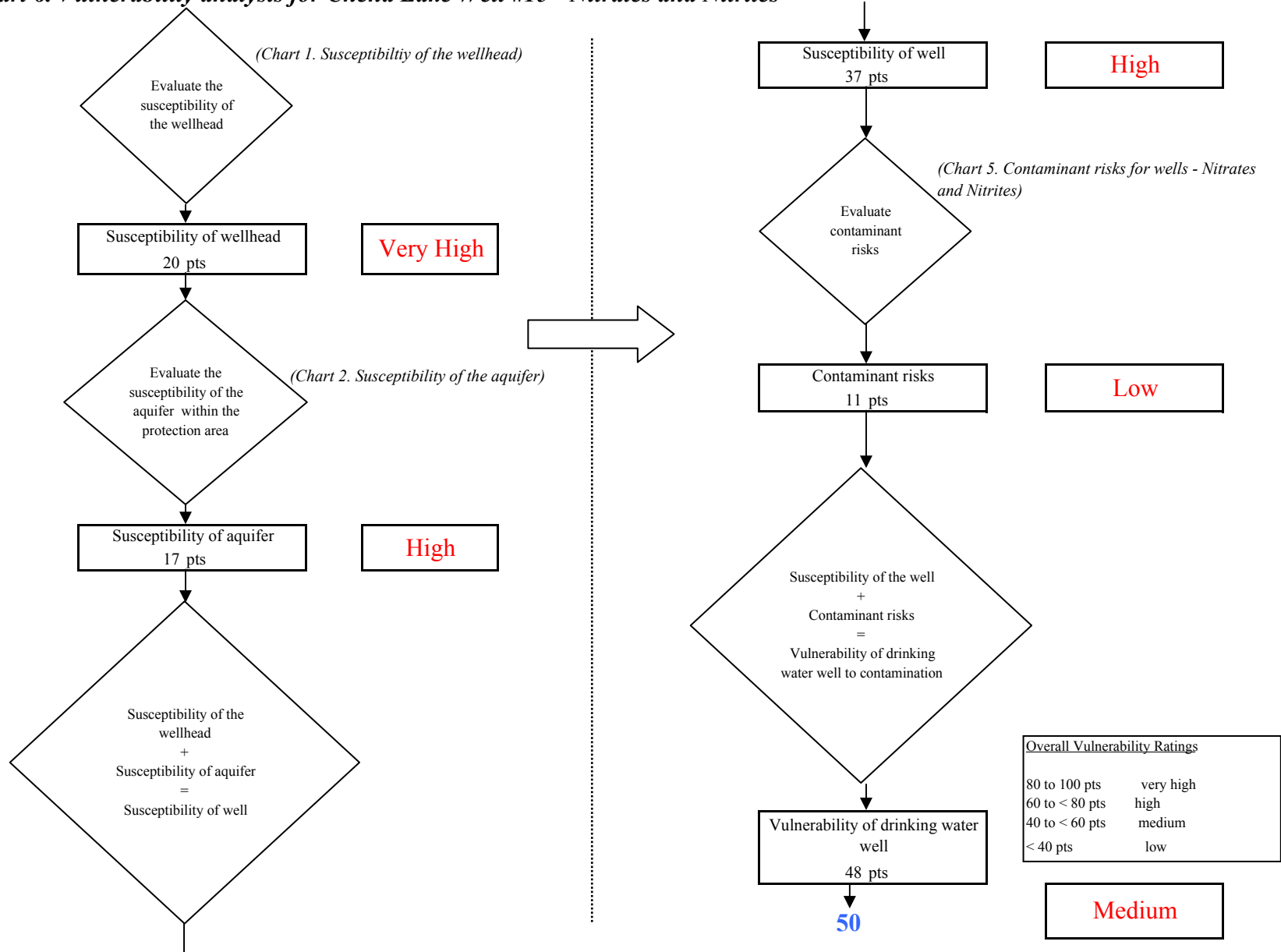
Chart 6. Vulnerability analysis for Chena Lake Well #15 - Nitrates and Nitrites
