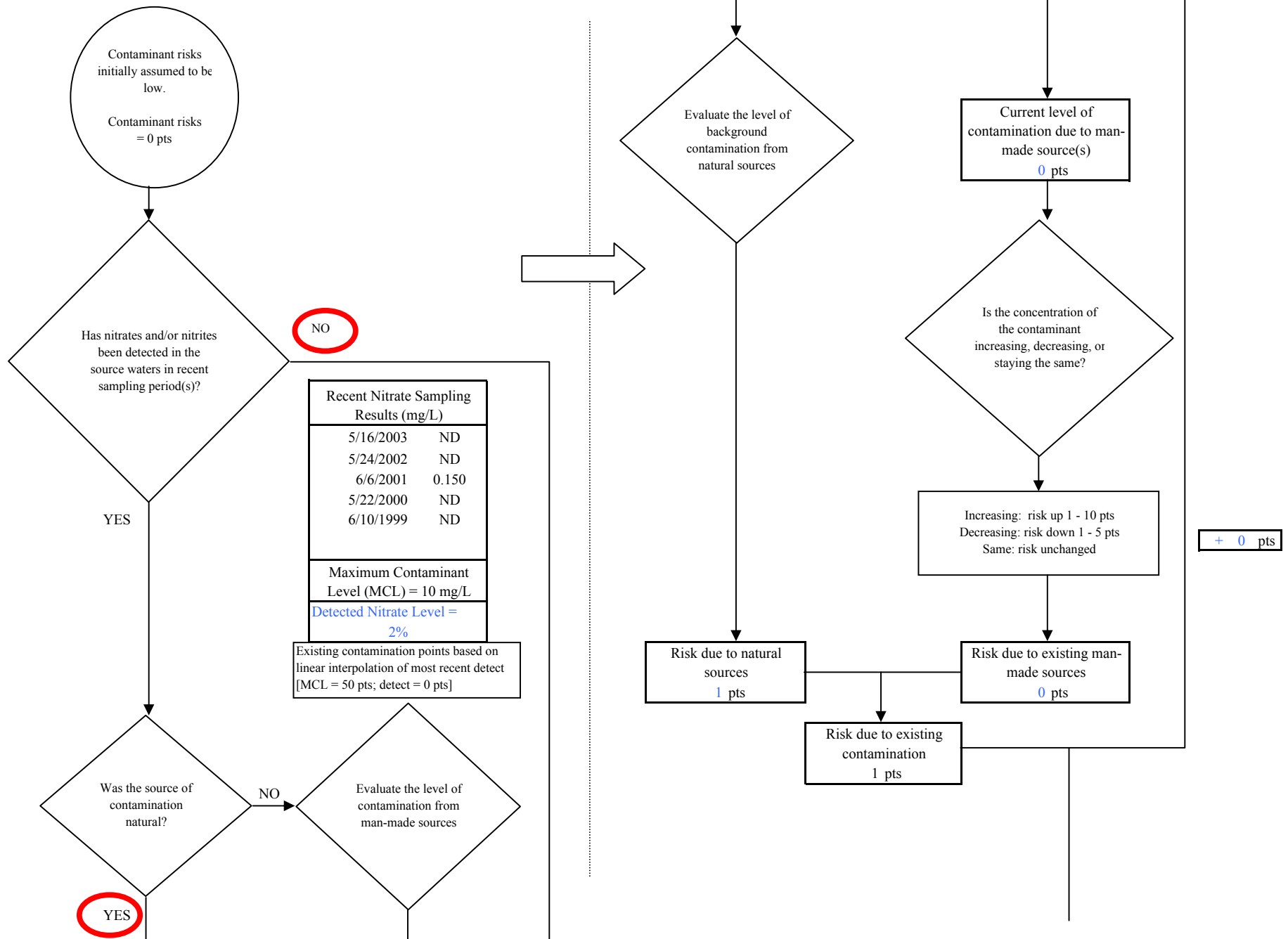
Chart 5. Contaminant risks for Chena Lake Well #15 - Nitrates and Nitrites
