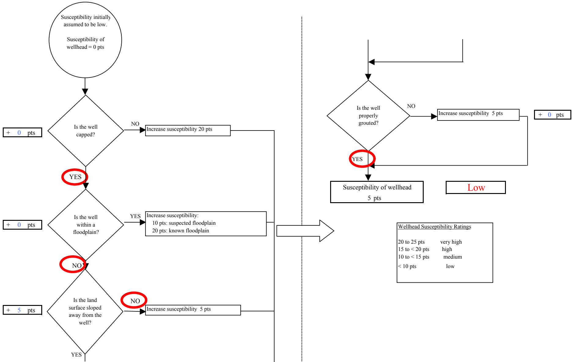
Chart 1. Susceptibility of the wellhead - Pizza Bella
