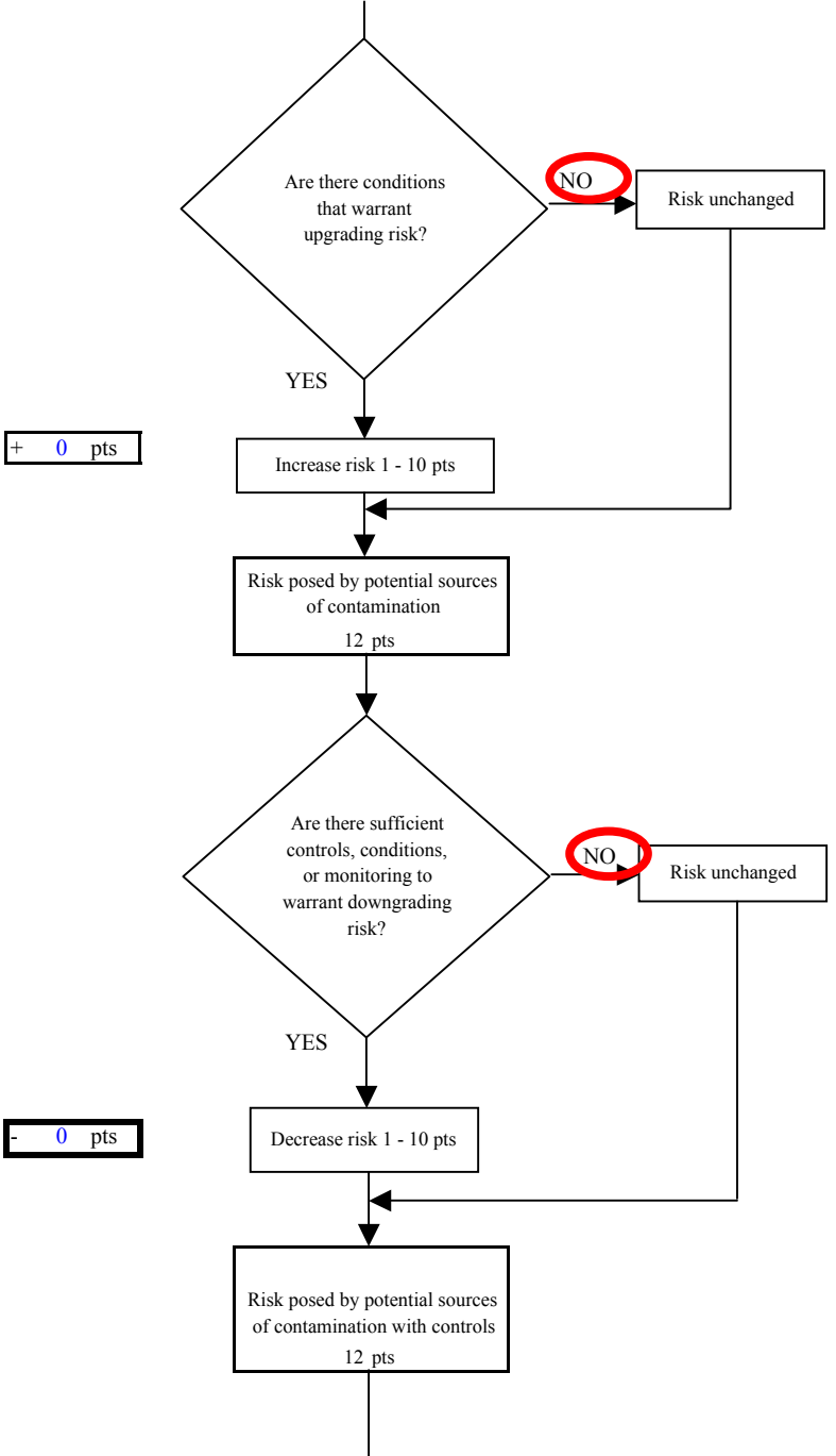
Chart 5. Contaminant risks for Pizza Bella - Nitrates and Nitrites
