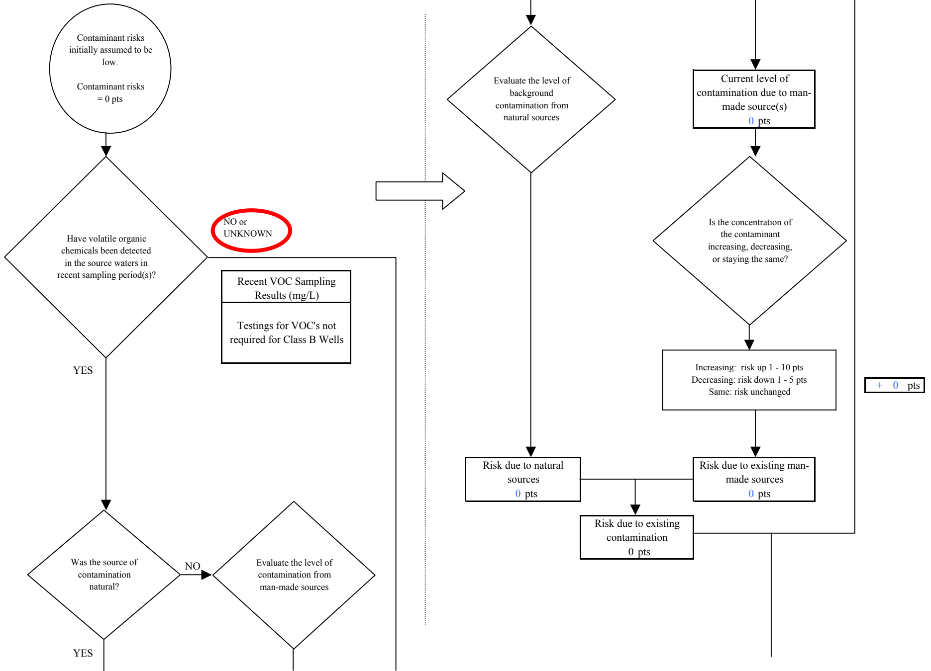
Chart 7. Contaminant risks for Delta / Clearwater Moose Lodge 911 - Volatile Organic Chemicals
