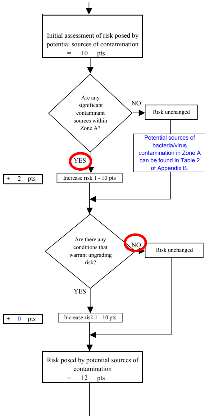
Chart 3. Contaminant risks for Delta / Clearwater Moose Lodge 911 - Bacteria & Viruses
