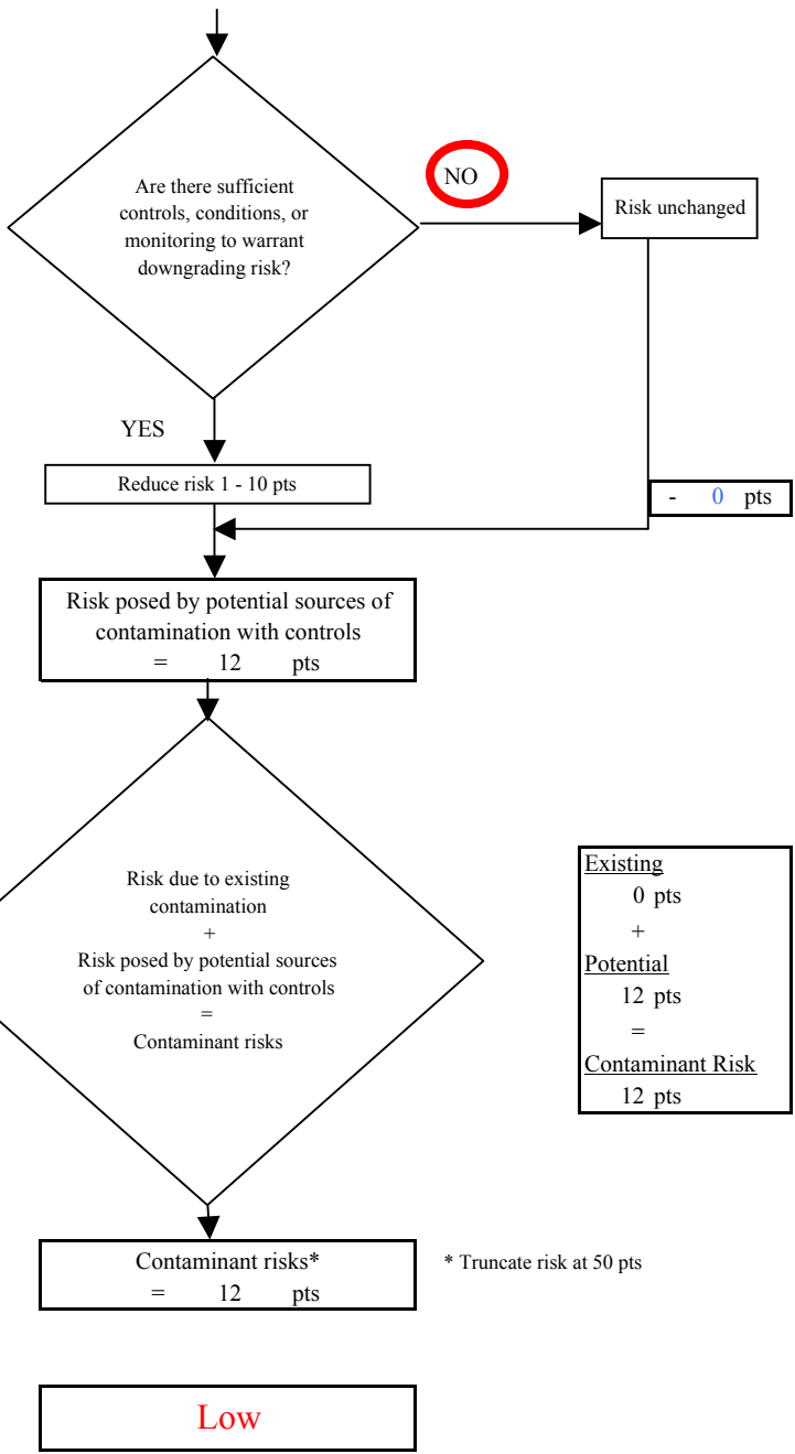
Chart 3. Contaminant risks for Delta / Clearwater Moose Lodge 911 - Bacteria & Viruses
