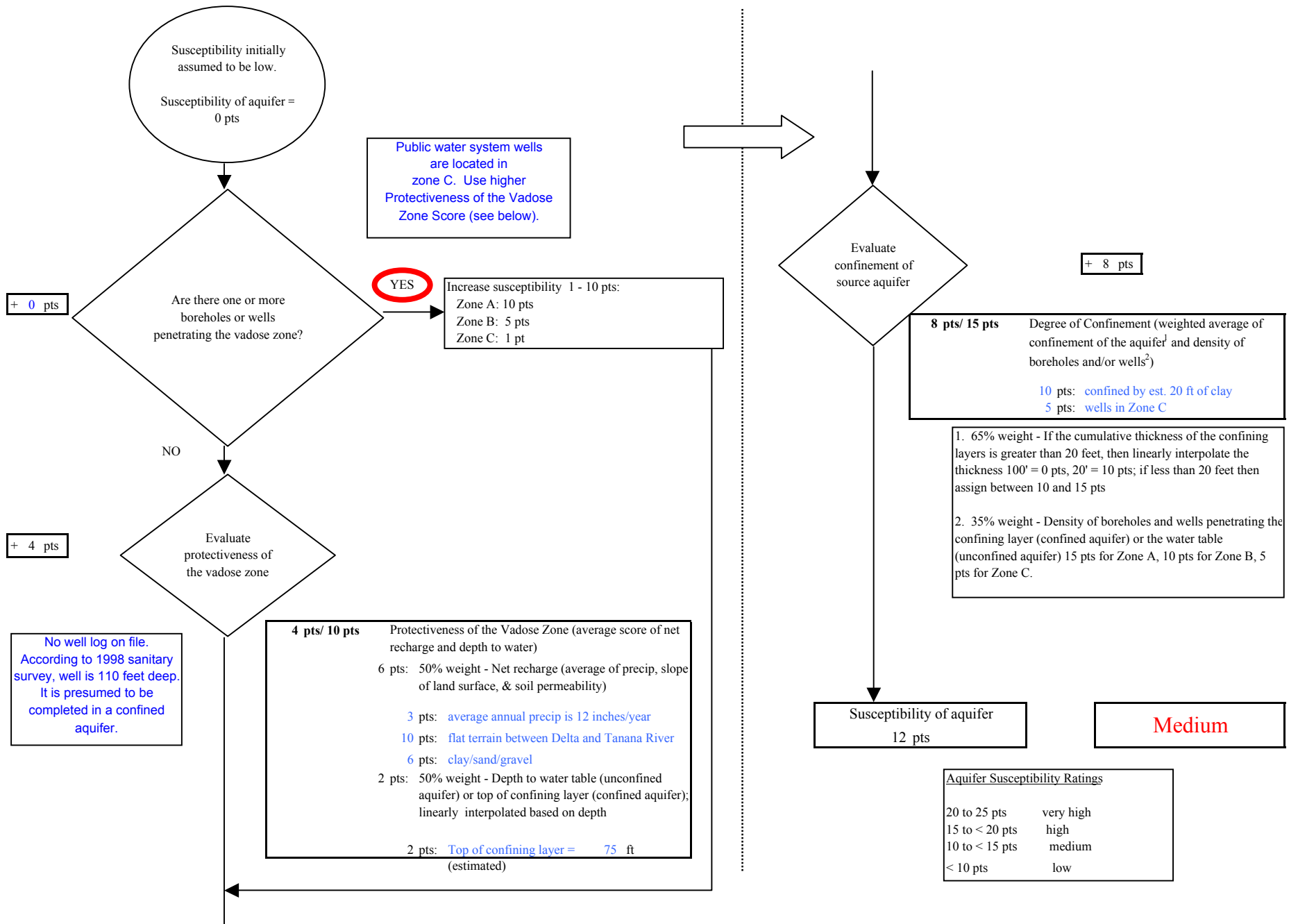
Chart 2. Susceptibility of the aquifer - Delta / Clearwater Moose Lodge 911
