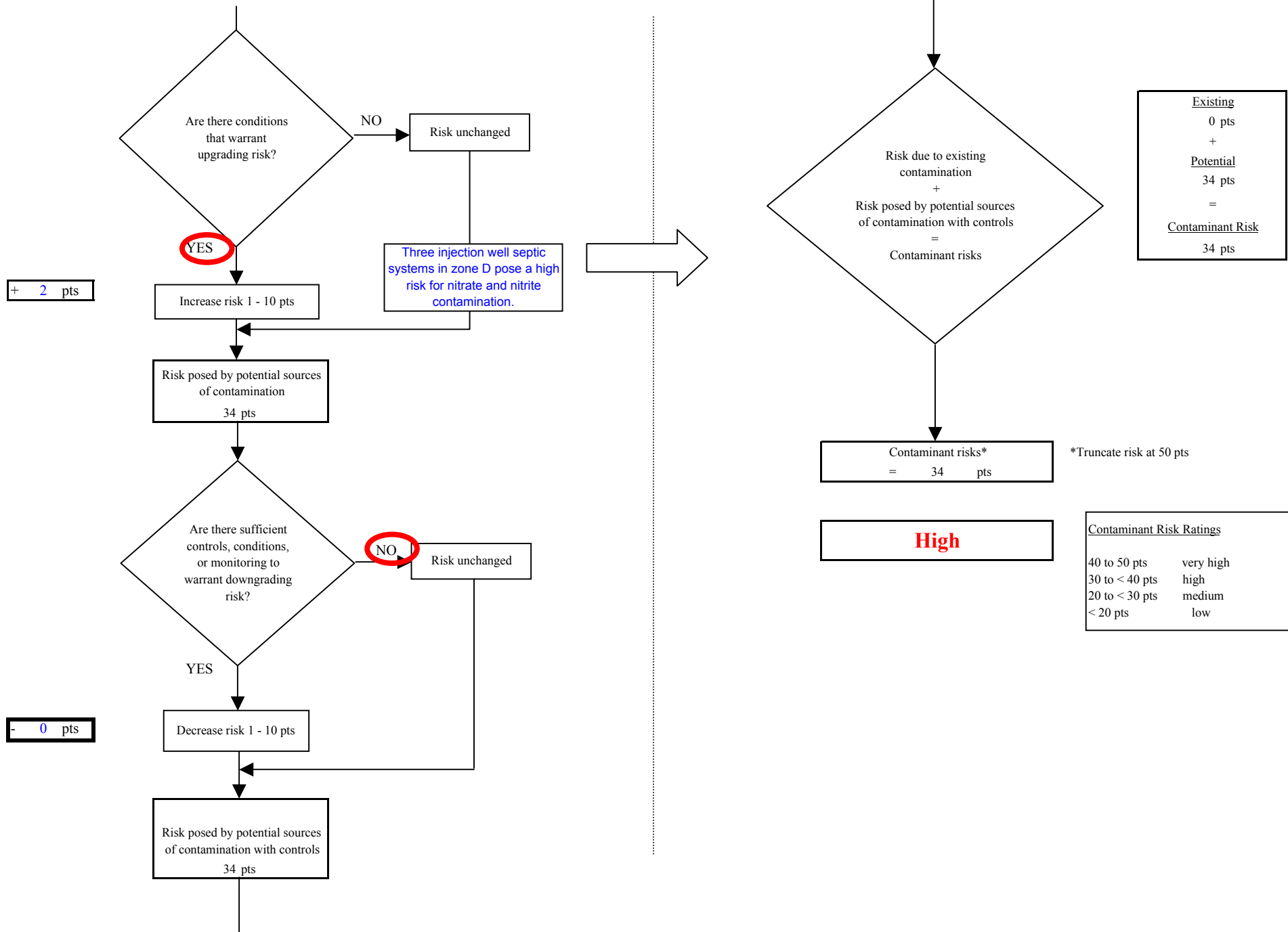
Chart 5. Contaminant risks for Delta / Clearwater Moose Lodge 911 - Nitrates and Nitrites
