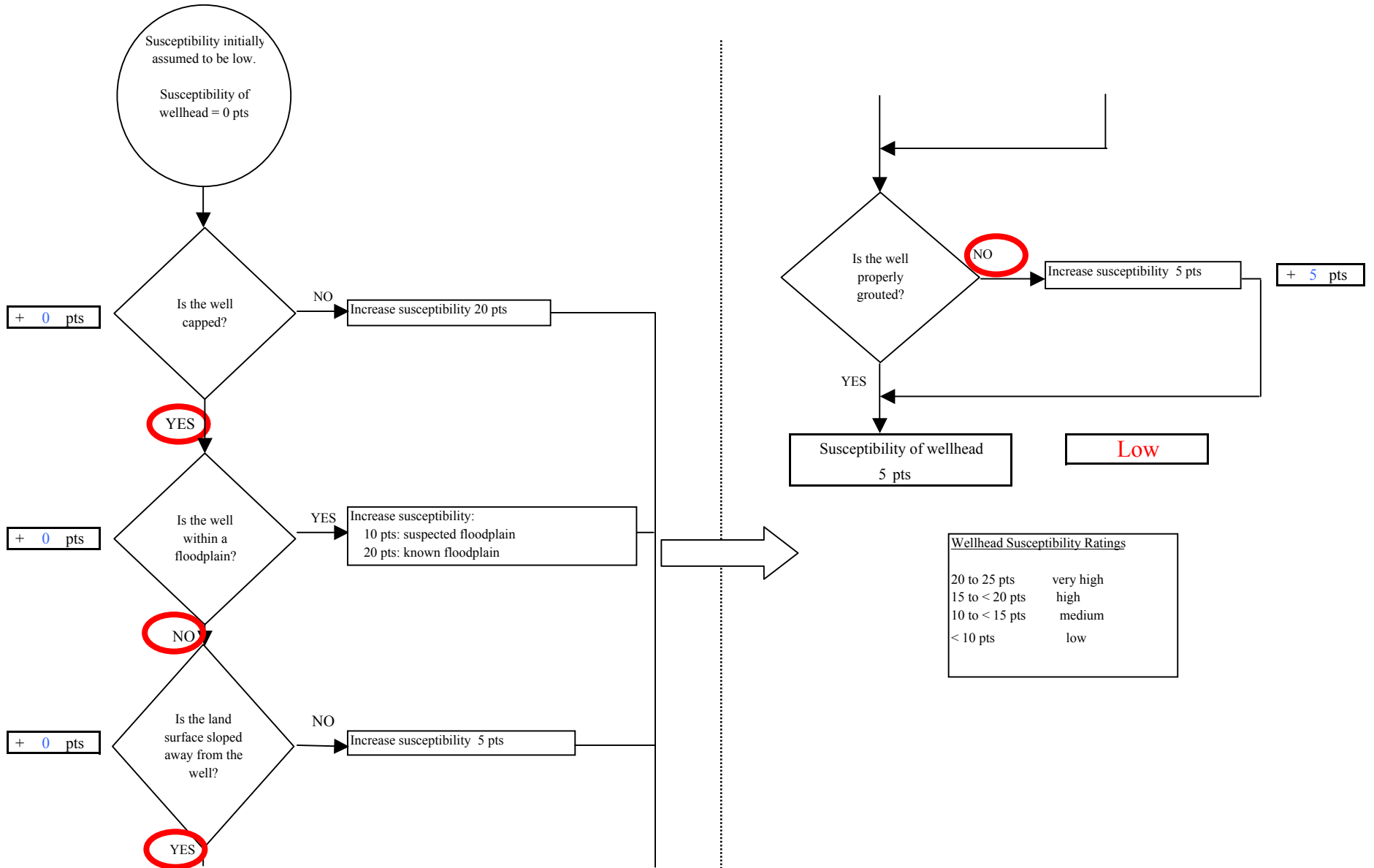
Chart 1. Susceptibility of the wellhead - Delta / Clearwater Moose Lodge 911
