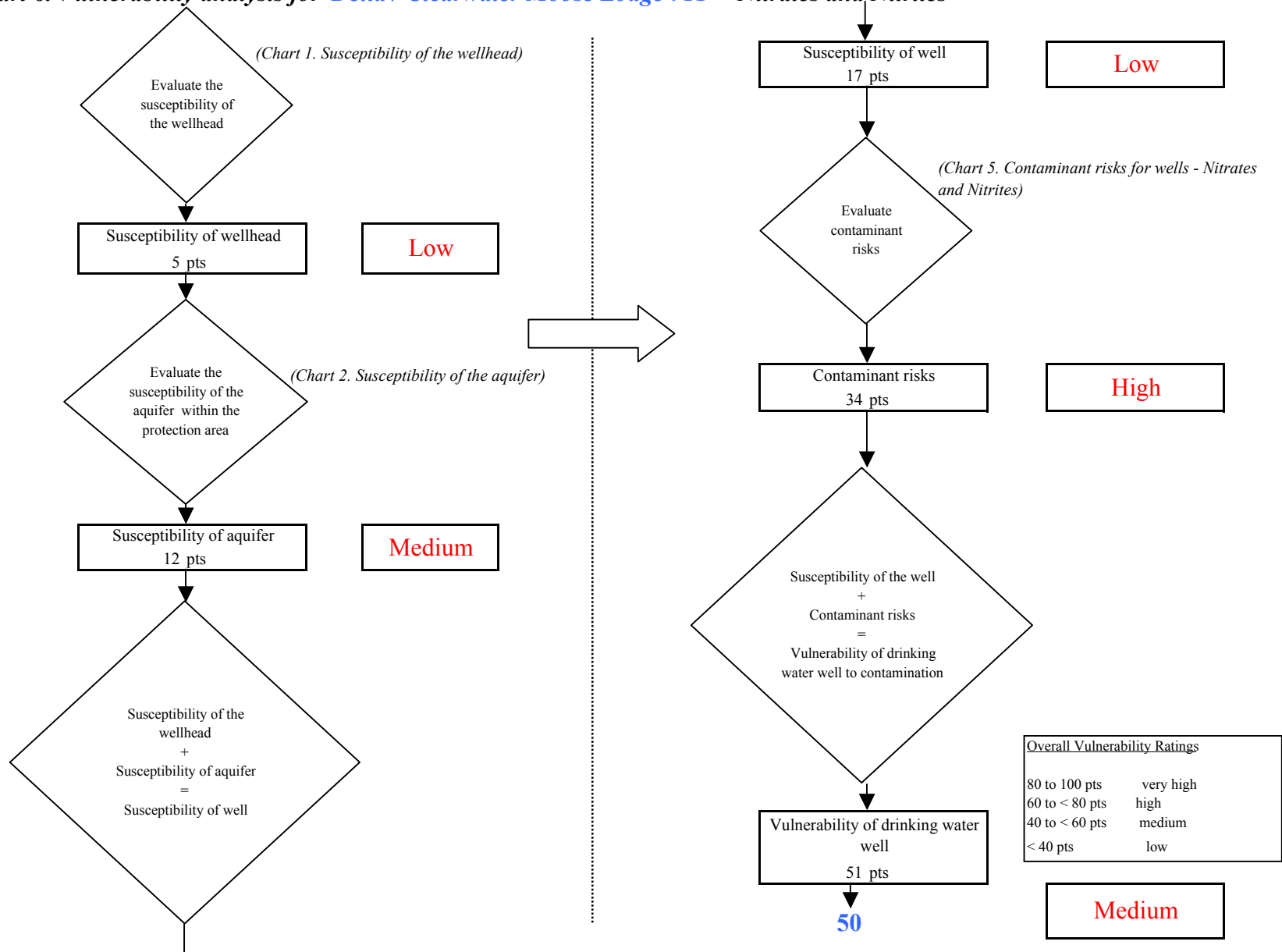
Chart 6. Vulnerability analysis for Delta / Clearwater Moose Lodge 911 - Nitrates and Nitrites
