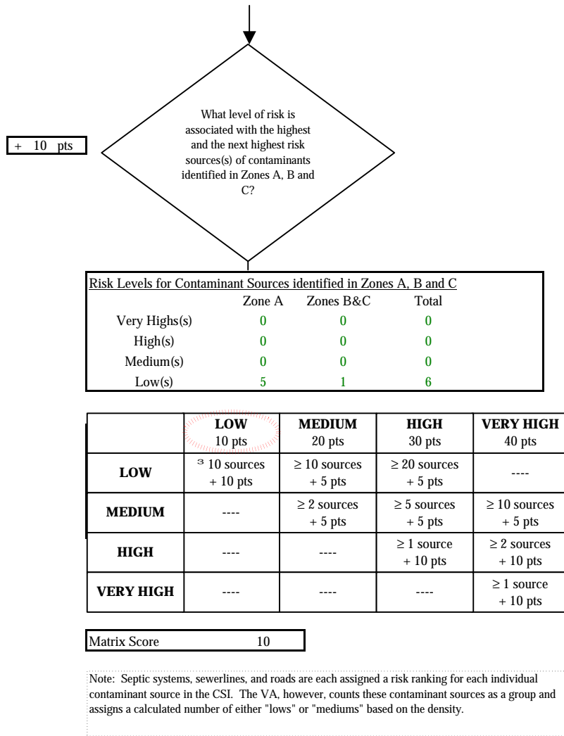
Chart 7. Contaminant risks for USFS Trail River Terrace (242296.001) - Volatile Organic Chemicals
