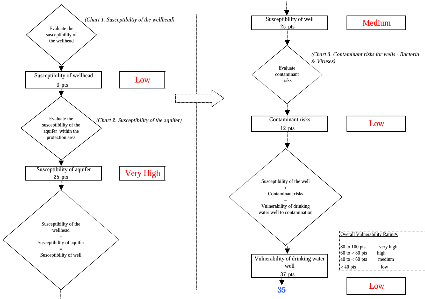
Chart 4. Vulnerability analysis for KNWR Visitors Center (248789.001) - Bacteria & Viruses
