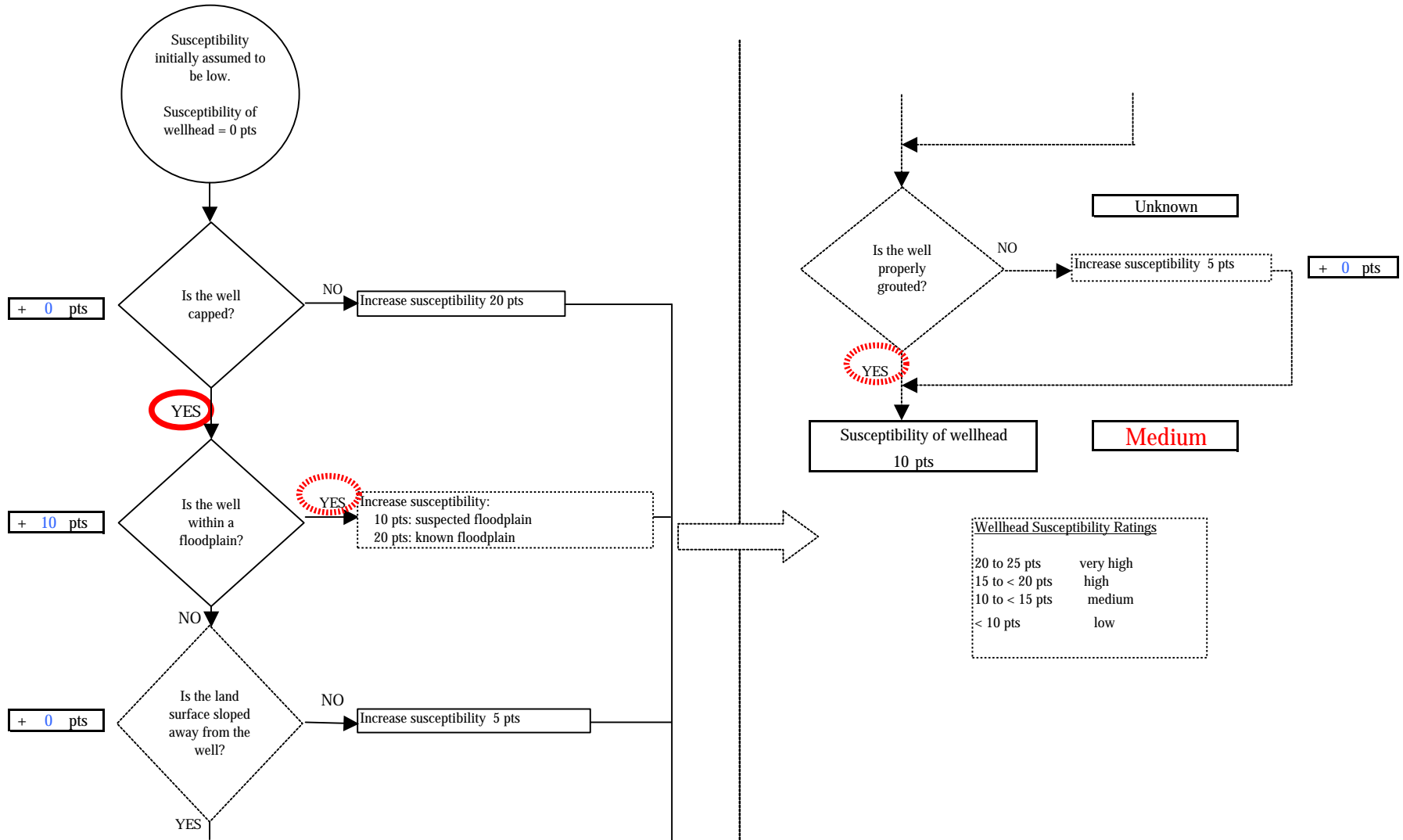
Chart 1. Susceptibility of the wellhead - USFS Crescent Creek Campground (240228.001)
