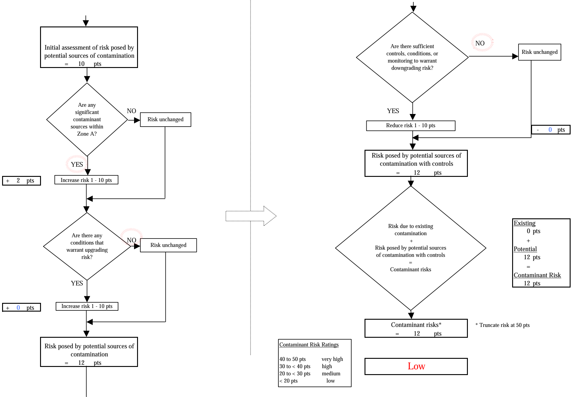
Chart 3. Contaminant risks for USFS Crescent Creek Campground (240228.001) - Bacteria & Viruses
