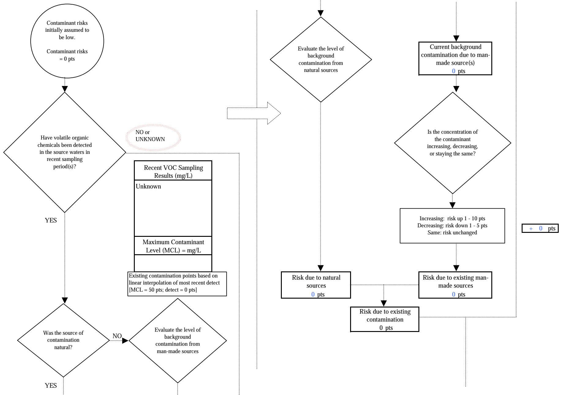
Chart 7. Contaminant risks for USFS Crescent Creek Campground (240228.001) - Volatile Organic Chemicals
