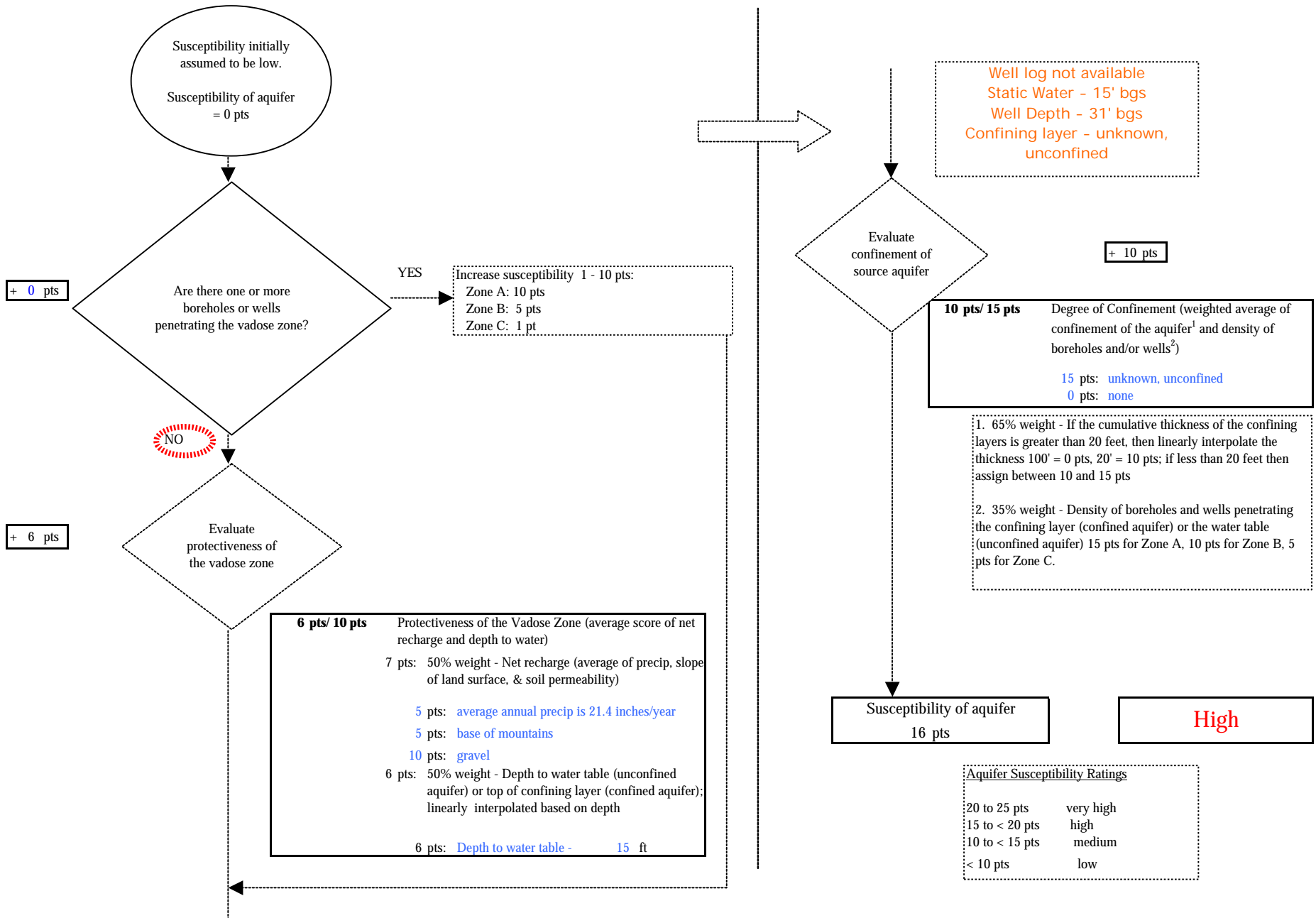
Chart 2. Susceptibility of the aquifer - USFS Crescent Creek Campground (240228.001)
