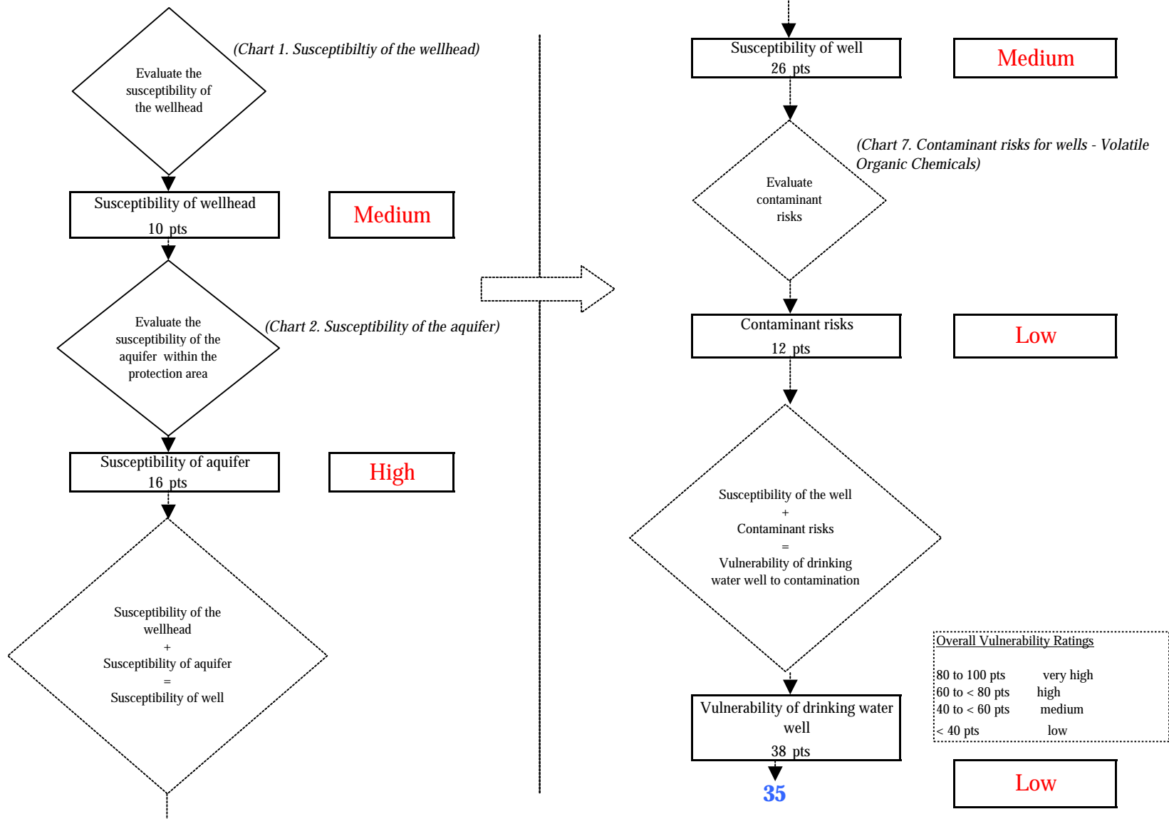
Chart 8. Vulnerability analysis for USFS Crescent Creek Campground (240228.001) - Volatile Organic Chemicals
