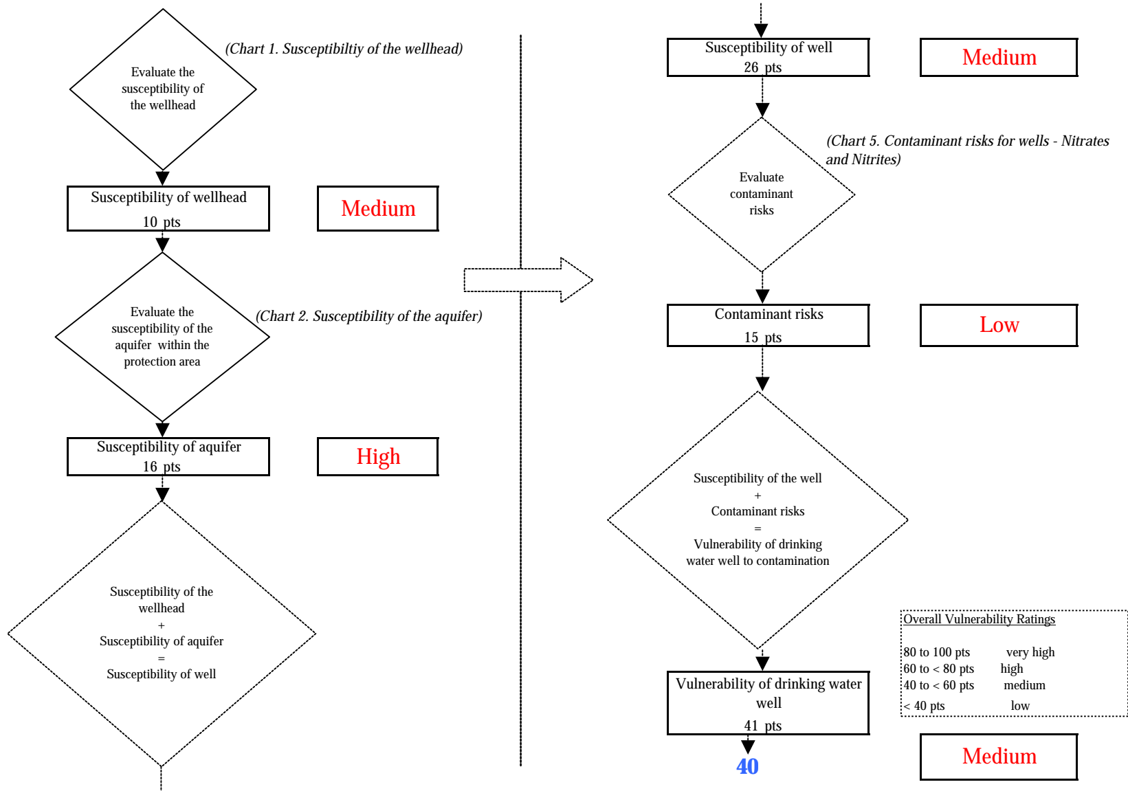
Chart 6. Vulnerability analysis for USFS Crescent Creek Campground (240228.001) - Nitrates and Nitrites
