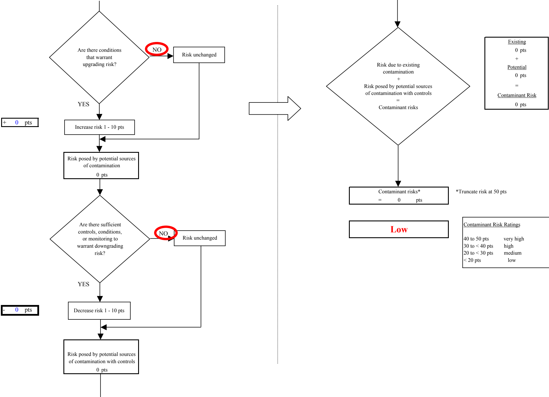
Chart 7. Contaminant risks for Cook Inlet Pipeline Drift River Terminal - Volatile Organic Chemicals
