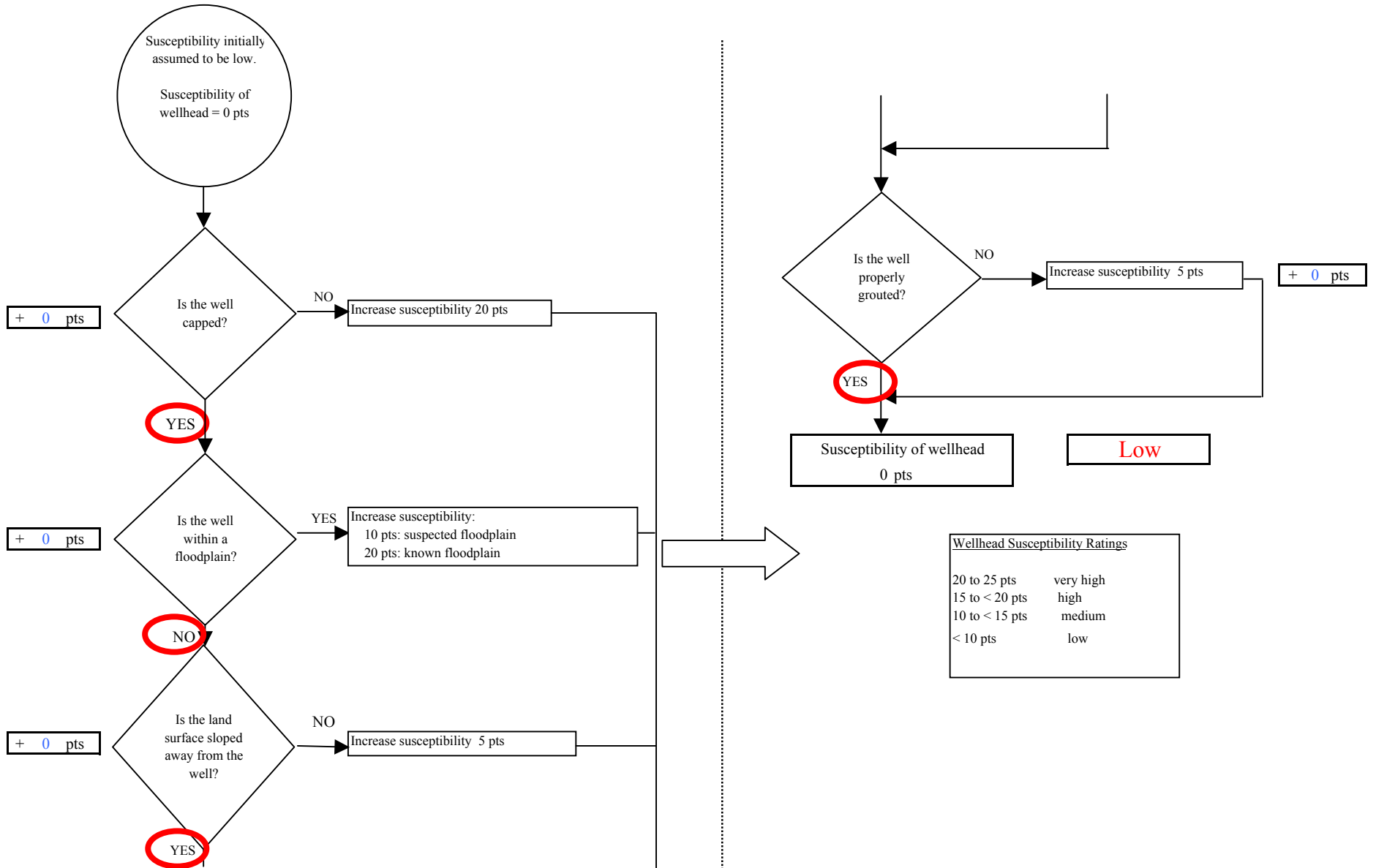
Chart 1. Susceptibility of the wellhead - Cook Inlet Pipeline Drift River Terminal
