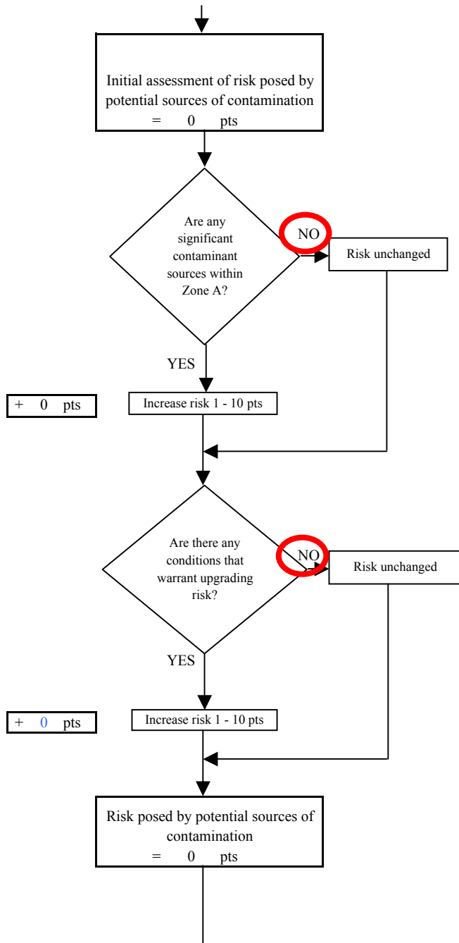
Chart 3. Contaminant risks for Cook Inlet Pipeline Drift River Terminal - Bacteria & Viruses
