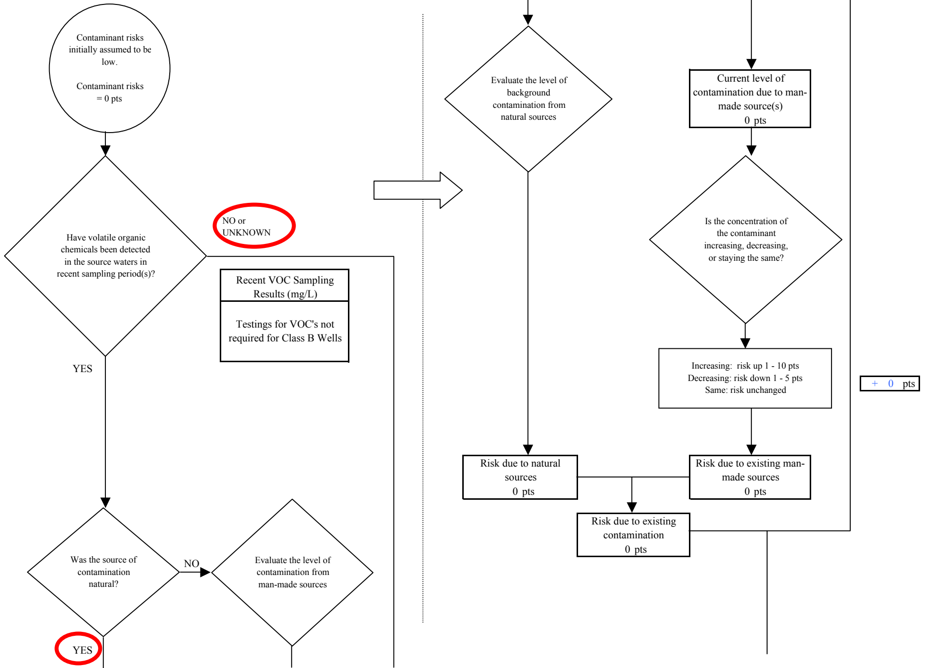
Chart 7. Contaminant risks for Cook Inlet Pipeline Drift River Terminal - Volatile Organic Chemicals
