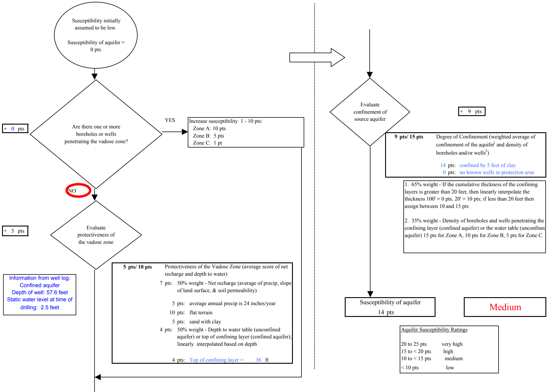
Chart 2. Susceptibility of the aquifer - Cook Inlet Pipeline Drift River Terminal
