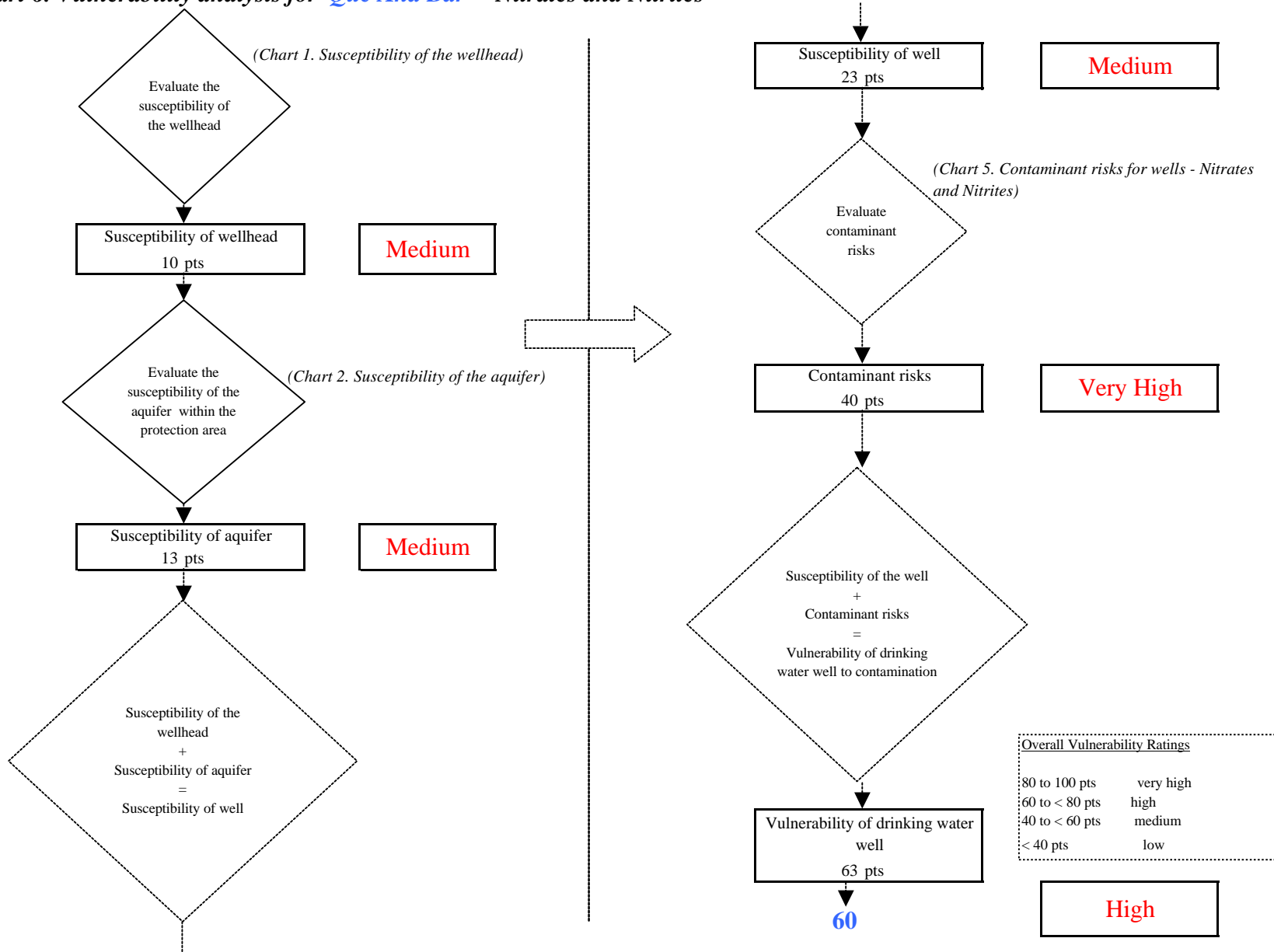
Chart 6. Vulnerability analysis for Que Ana Bar - Nitrates and Nitrites
