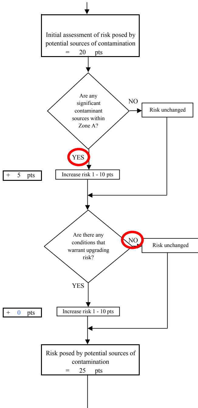
Chart 3. Contaminant risks for Troll Knoll Subdivision - Bacteria & Viruses
