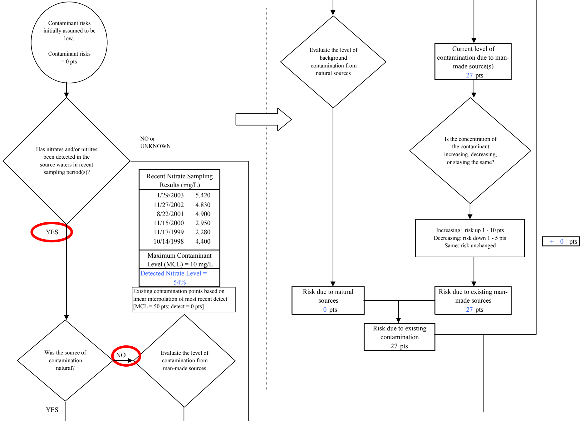
Chart 5. Contaminant risks for Troll Knoll Subdivision - Nitrates and Nitrites
