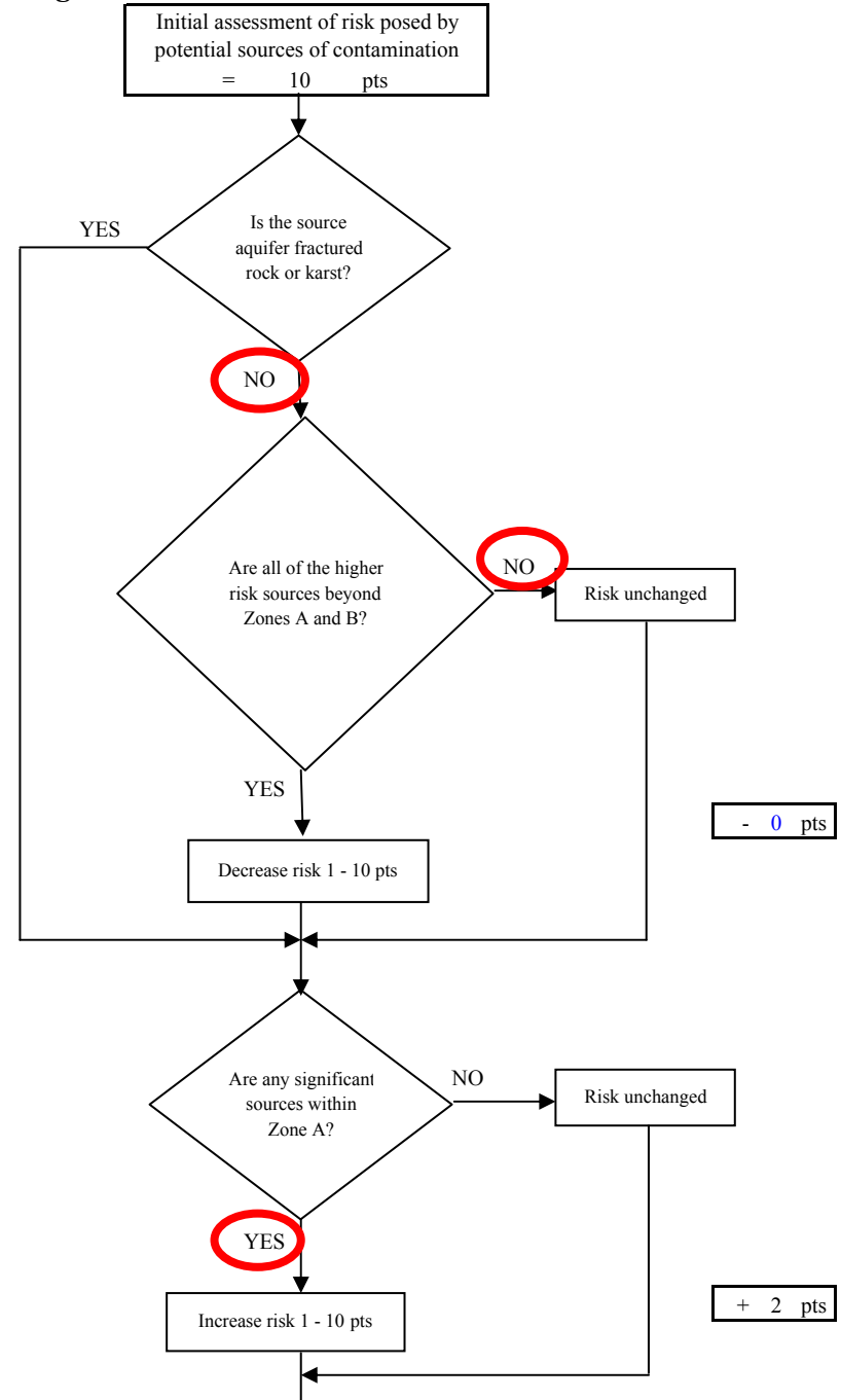
Chart 9. Contaminant risks for Troll Knoll Subdivision - Heavy Metals, Cyanide and Other Inorganic Chemicals
