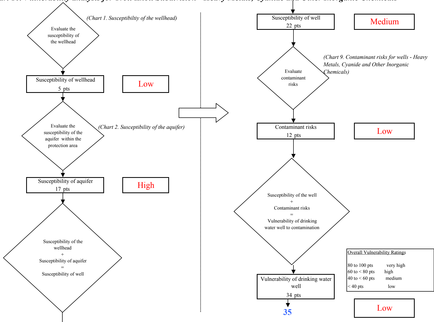
Chart 10. Vulnerability analysis for Troll Knoll Subdivision - Heavy Metals, Cyanide and Other Inorganic Chemicals
