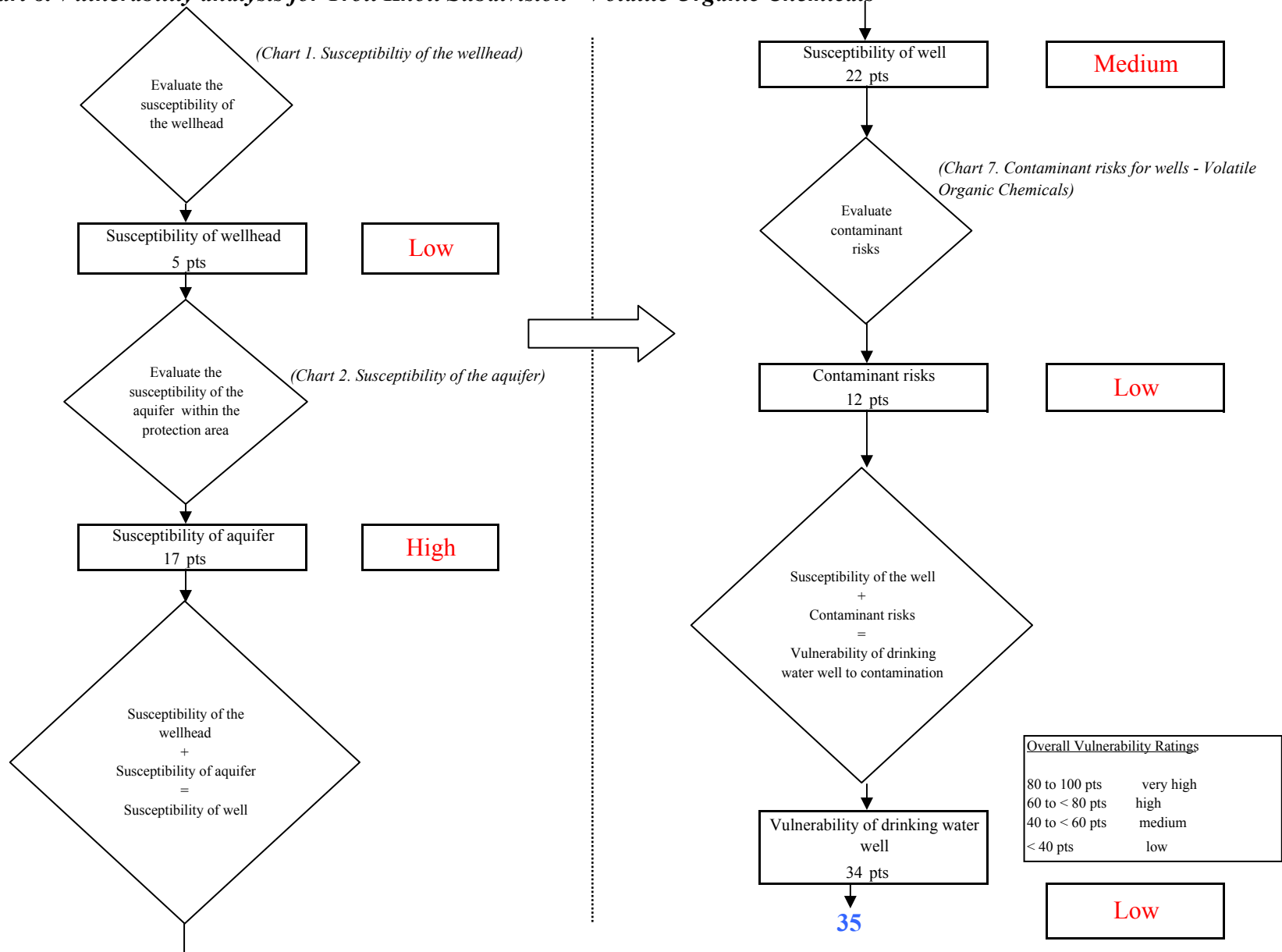
Chart 8. Vulnerability analysis for Troll Knoll Subdivision - Volatile Organic Chemicals
