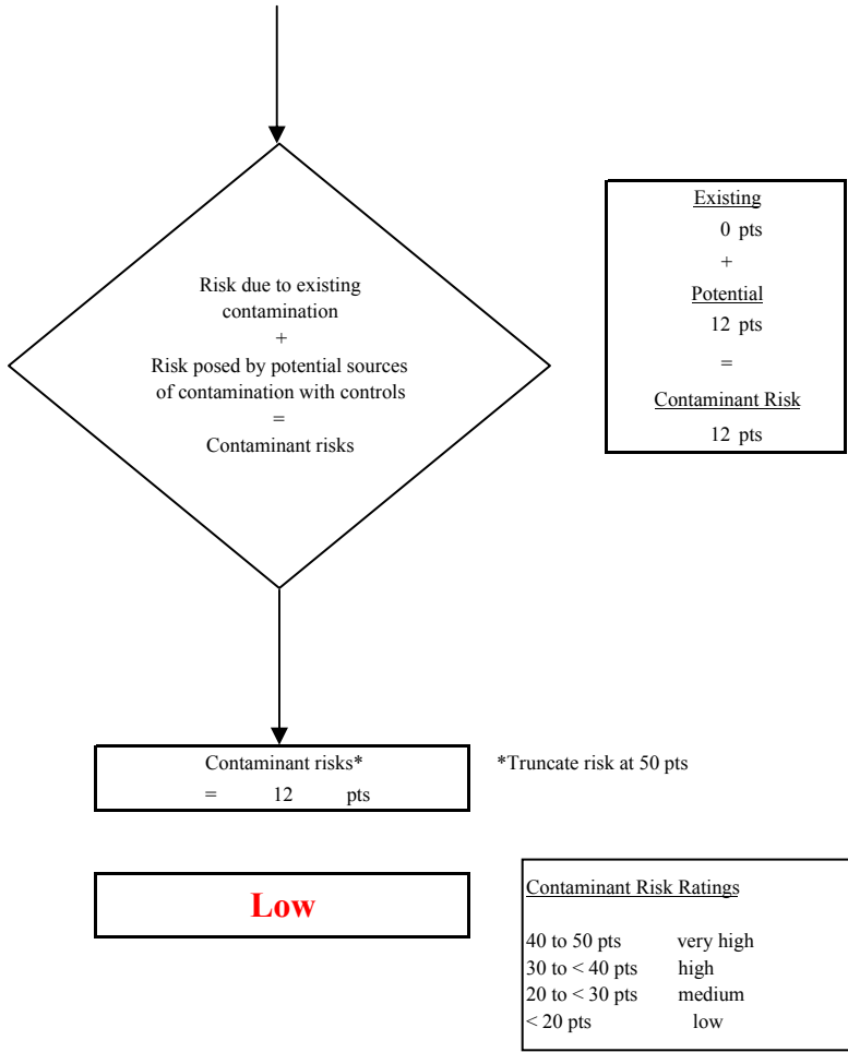
Chart 7. Contaminant risks for Troll Knoll Subdivision - Volatile Organic Chemicals
