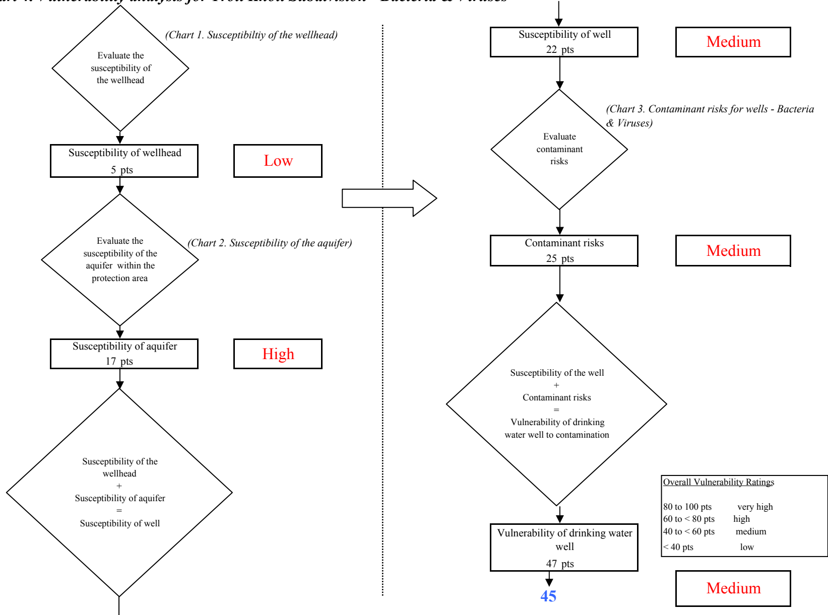
Chart 4. Vulnerability analysis for Troll Knoll Subdivision - Bacteria & Viruses
