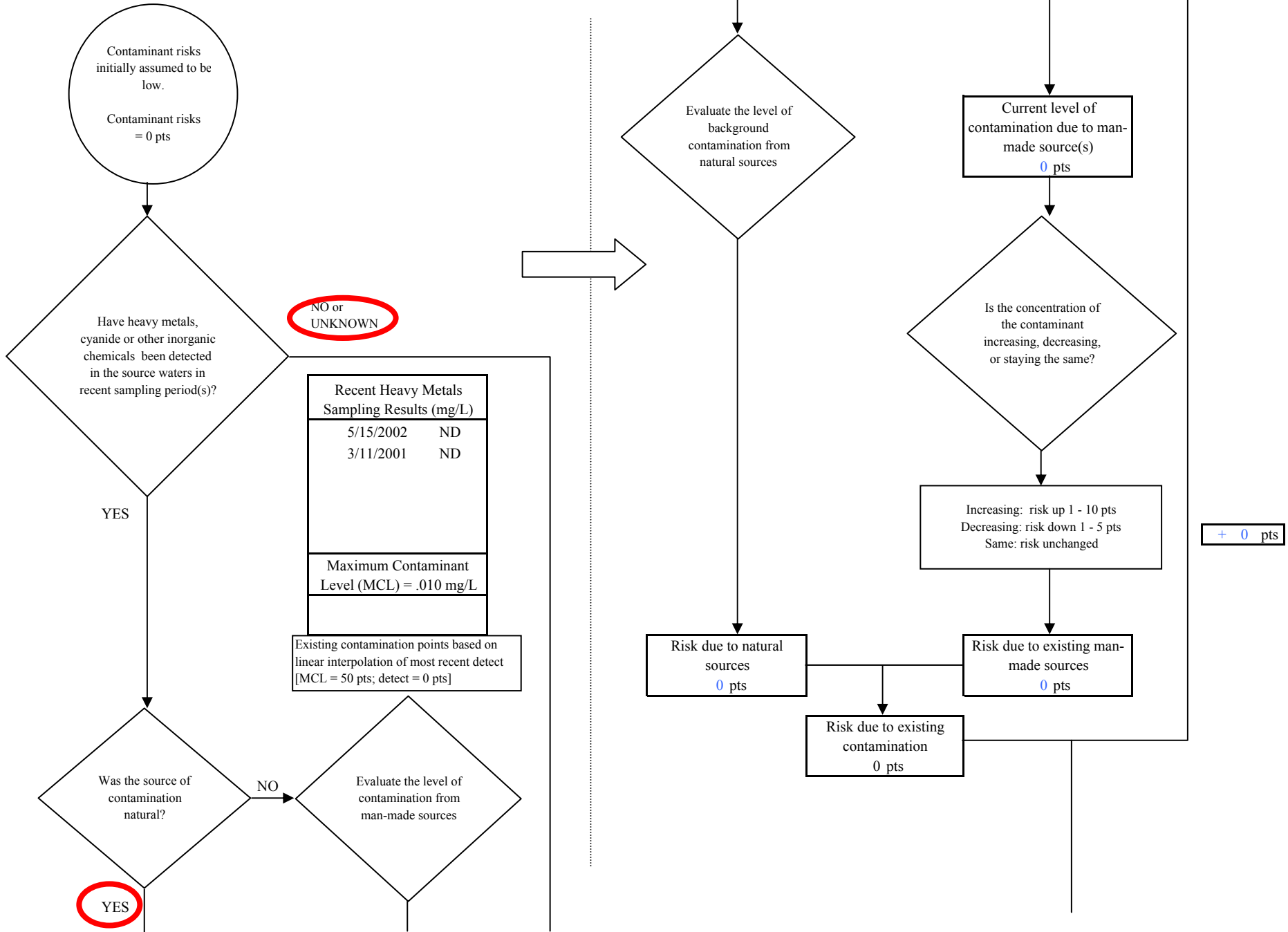
Chart 9. Contaminant risks for Troll Knoll Subdivision - Heavy Metals, Cyanide and Other Inorganic Chemicals
