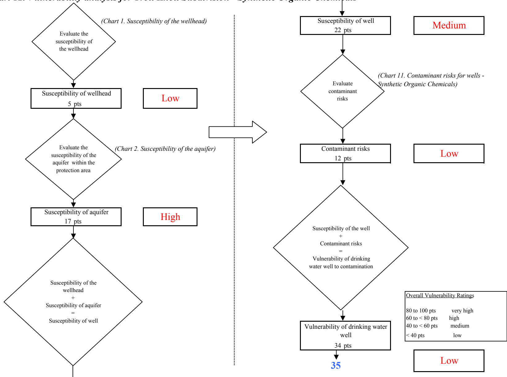
Chart 12. Vulnerability analysis for Troll Knoll Subdivision - Synthetic Organic Chemicals
