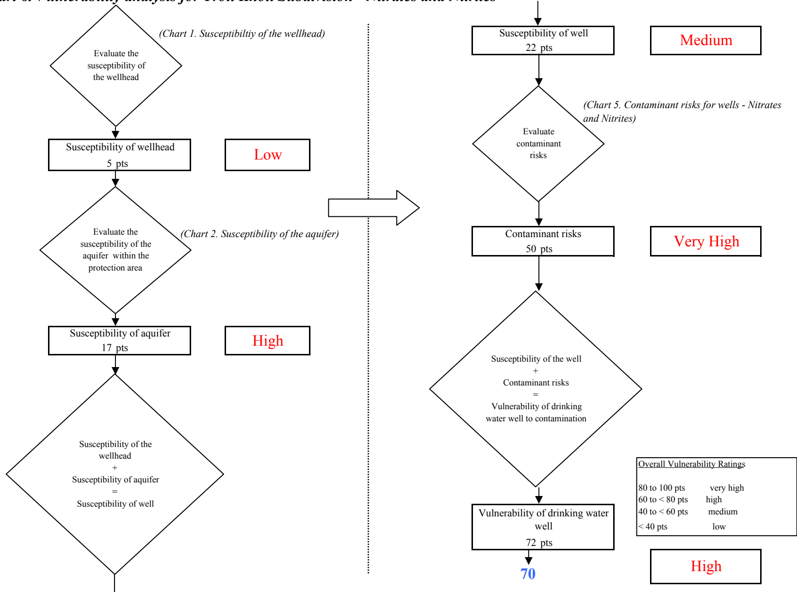
Chart 6. Vulnerability analysis for Troll Knoll Subdivision - Nitrates and Nitrites
