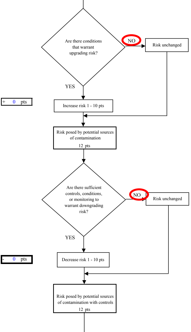
Chart 7. Contaminant risks for Troll Knoll Subdivision - Volatile Organic Chemicals
