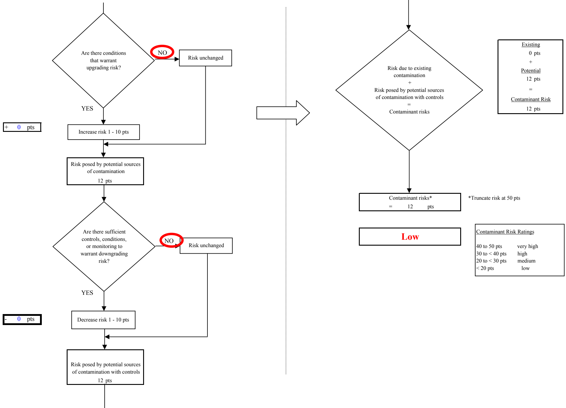
Chart 9. Contaminant risks for Troll Knoll Subdivision - Heavy Metals, Cyanide and Other Inorganic Chemicals
