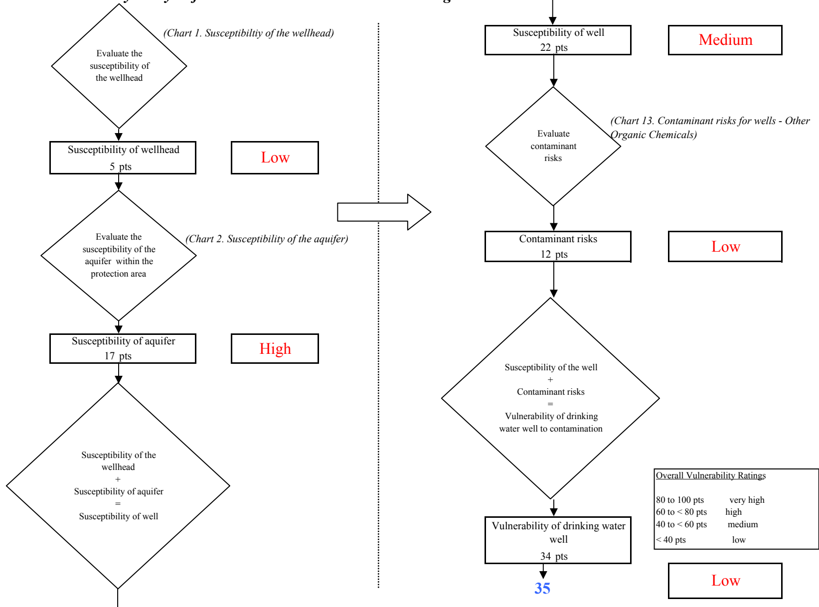
Chart 14. Vulnerability analysis for Troll Knoll Subdivision - Other Organic Chemicals
