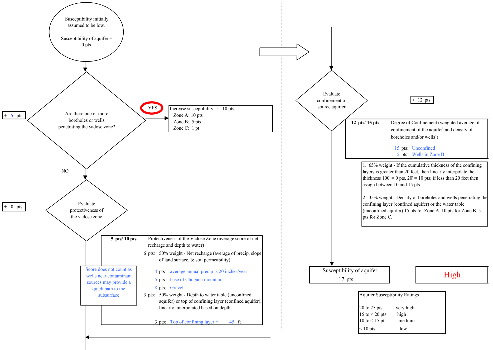
Chart 2. Susceptibility of the aquifer - Troll Knoll Subdivision
