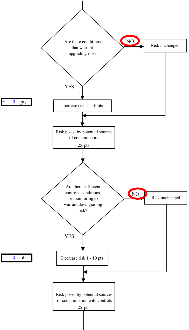
Chart 5. Contaminant risks for Troll Knoll Subdivision - Nitrates and Nitrites
