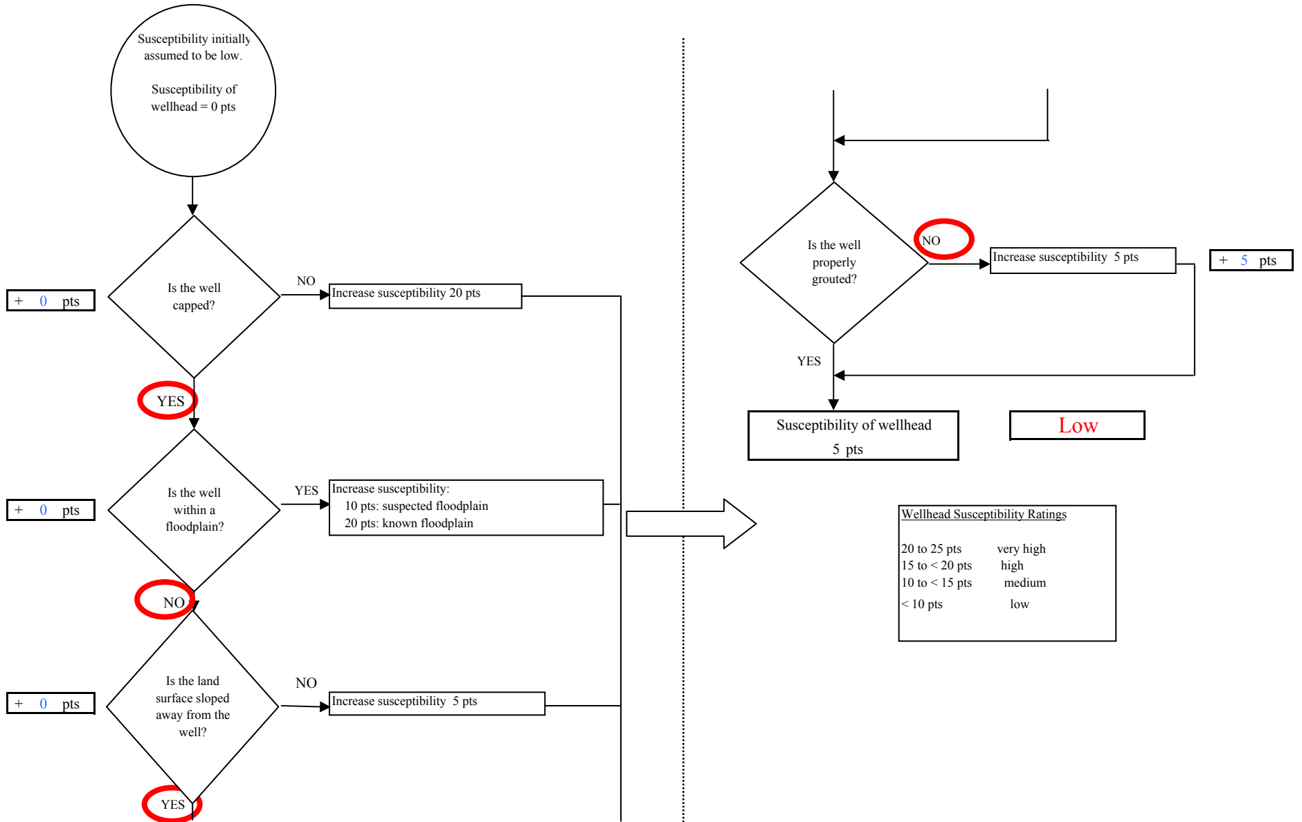
Chart 1. Susceptibility of the wellhead - Troll Knoll Subdivision
