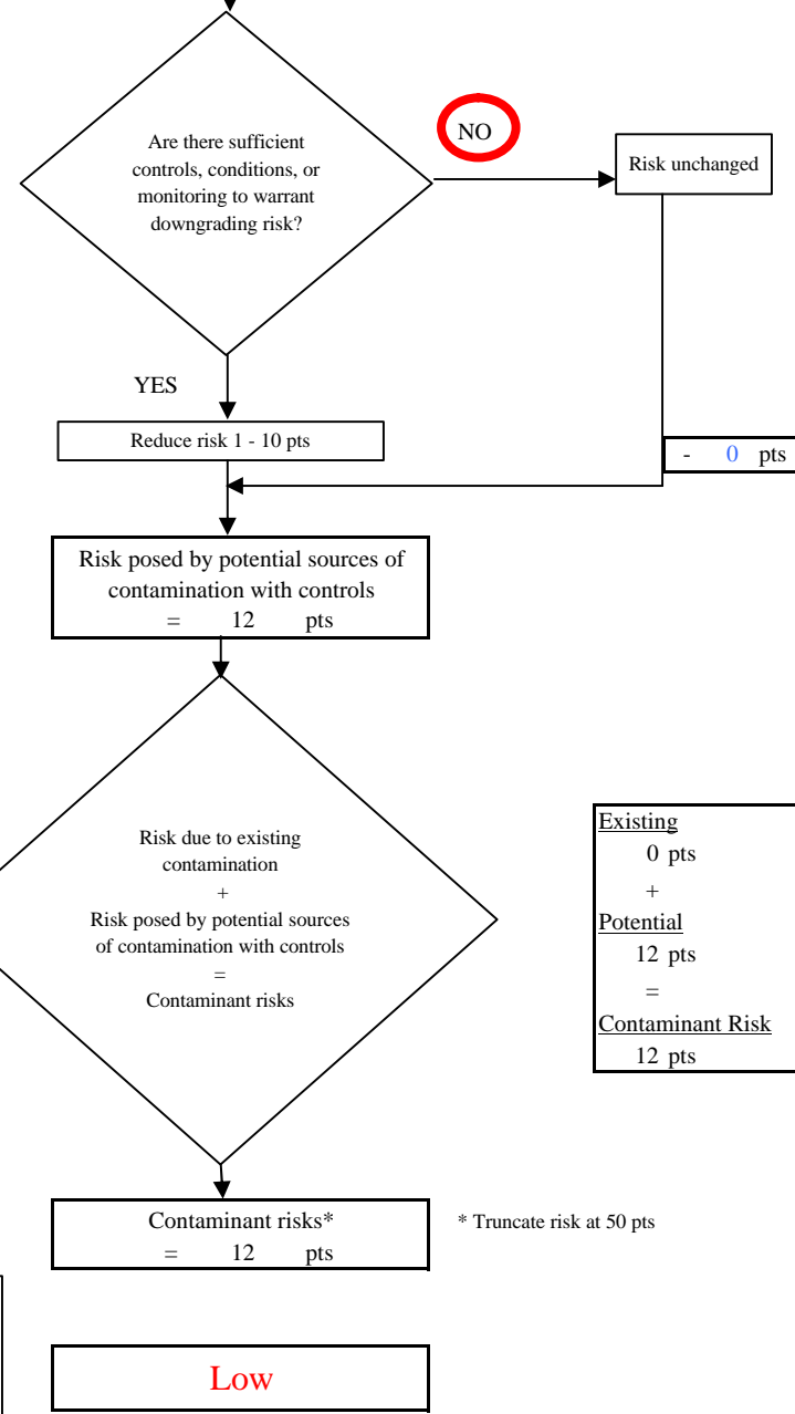
Chart 3. Contaminant Risks for Sheep Mountain Lodge - Bacteria & Viruses
