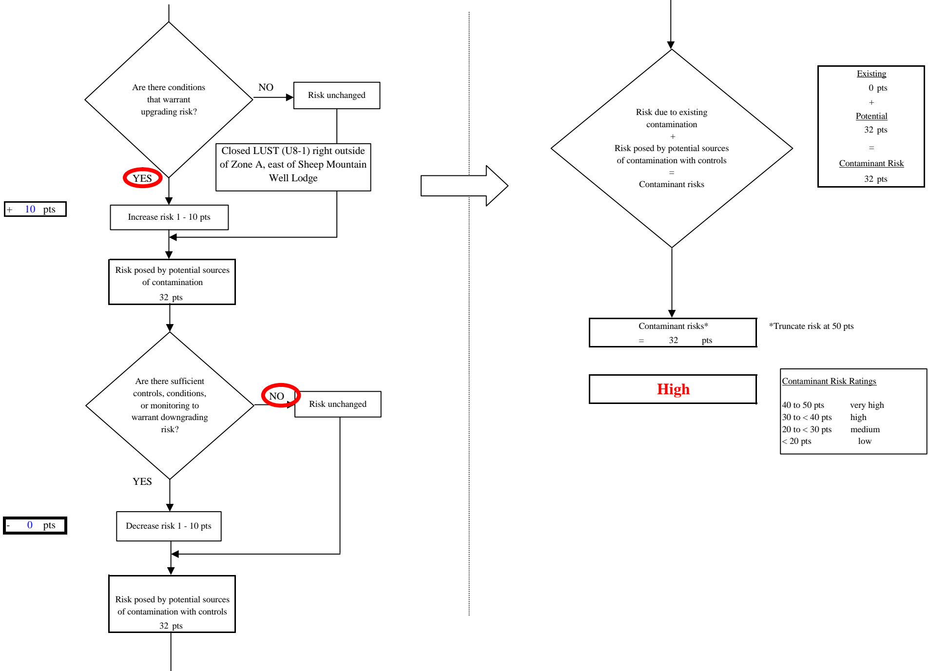
Chart 7. Contaminant Risks for Sheep Mountain Lodge - Volatile Organic Chemicals
