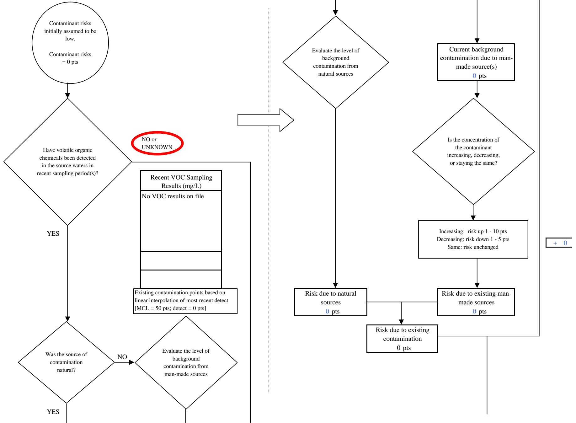
Chart 7. Contaminant Risks for Sheep Mountain Lodge - Volatile Organic Chemicals
