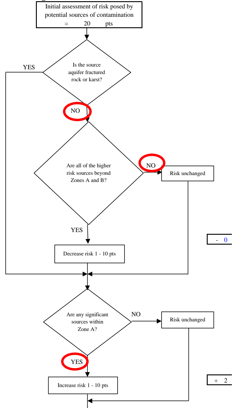
Chart 7. Contaminant Risks for Sheep Mountain Lodge - Volatile Organic Chemicals
