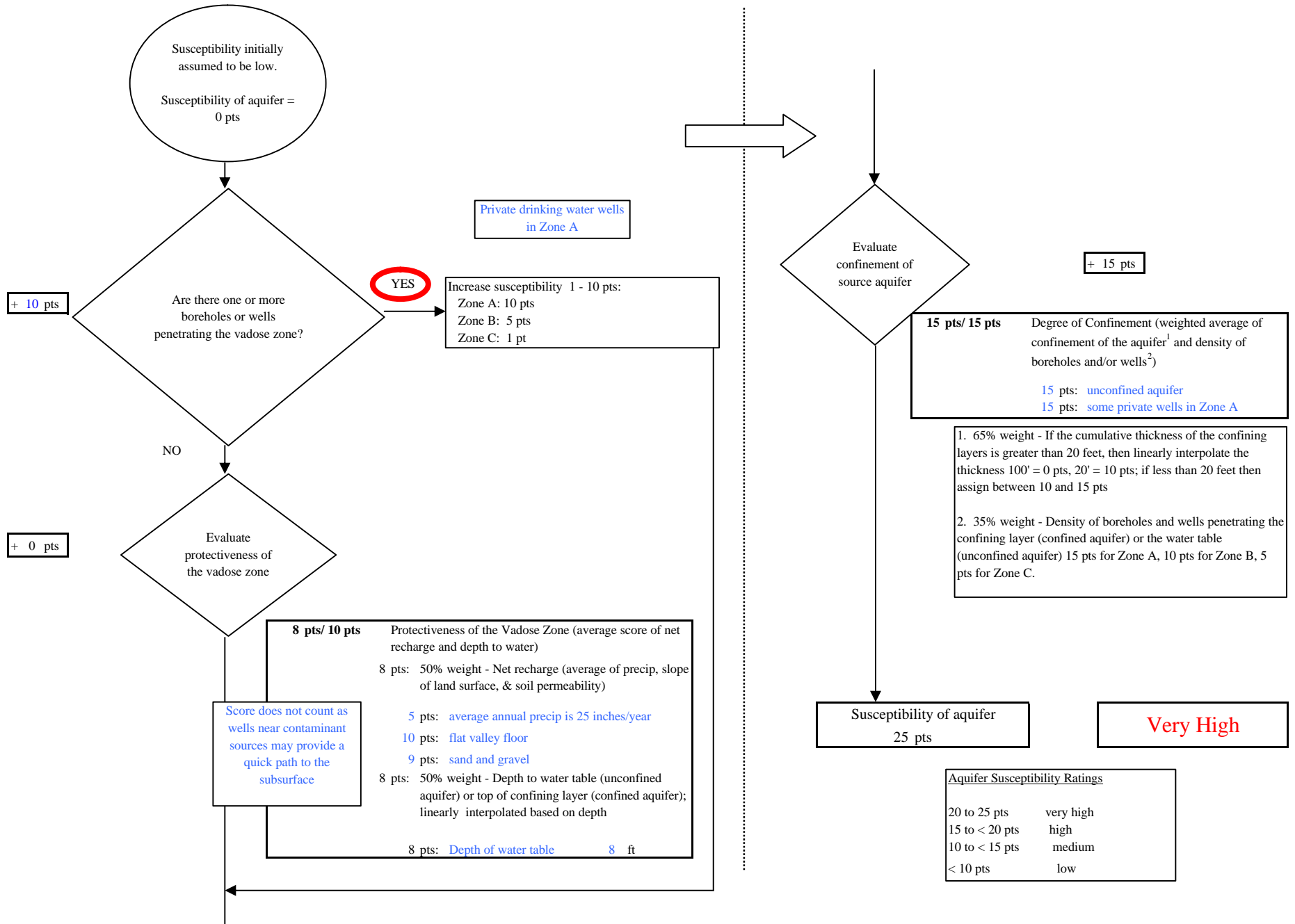
Chart 2. Susceptibility of the Aquifer - Sheep Mountain Lodge
