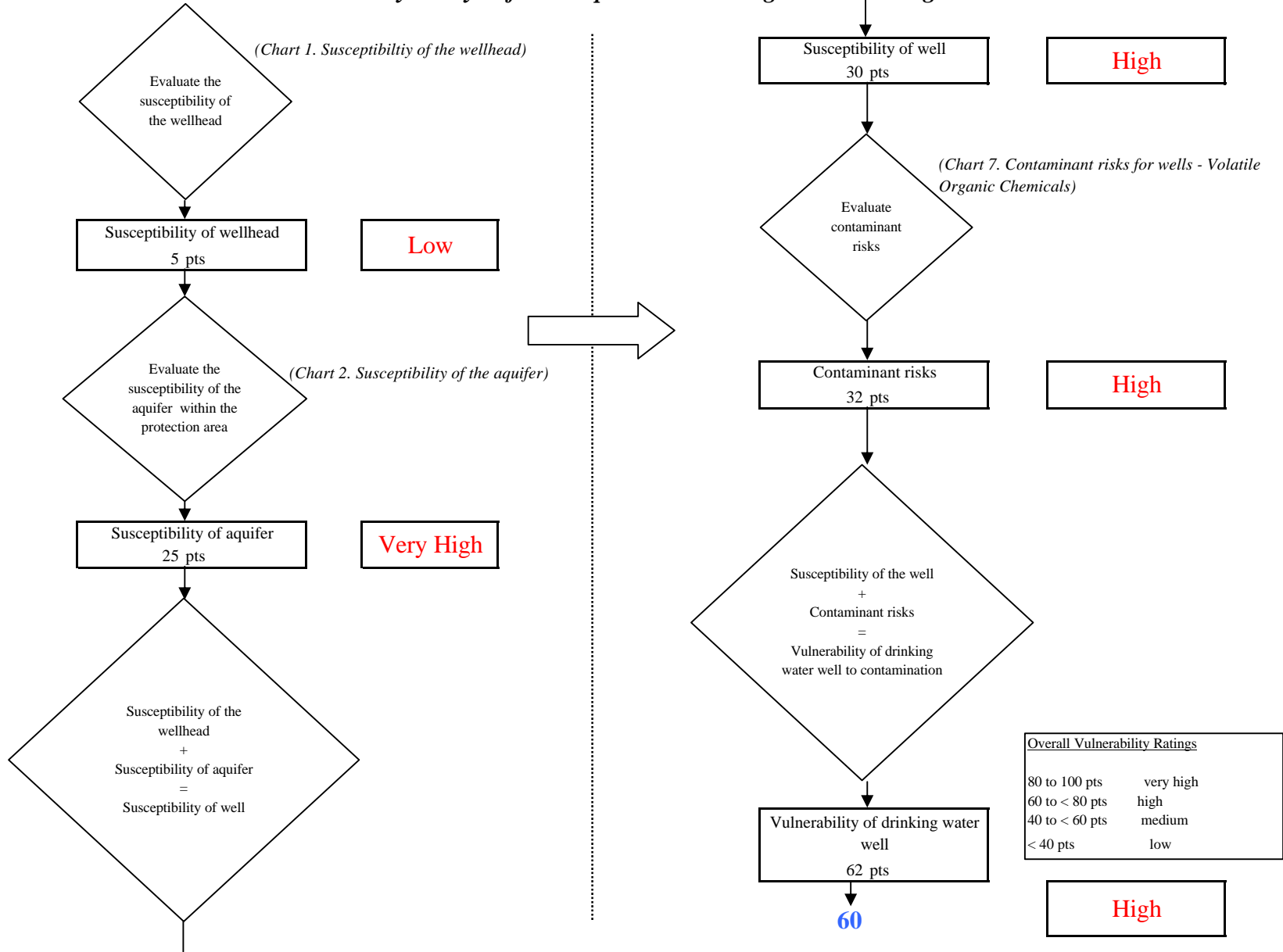
Chart 8. Vulnerability Analysis for Sheep Mountain Lodge - Volatile Organic Chemicals
