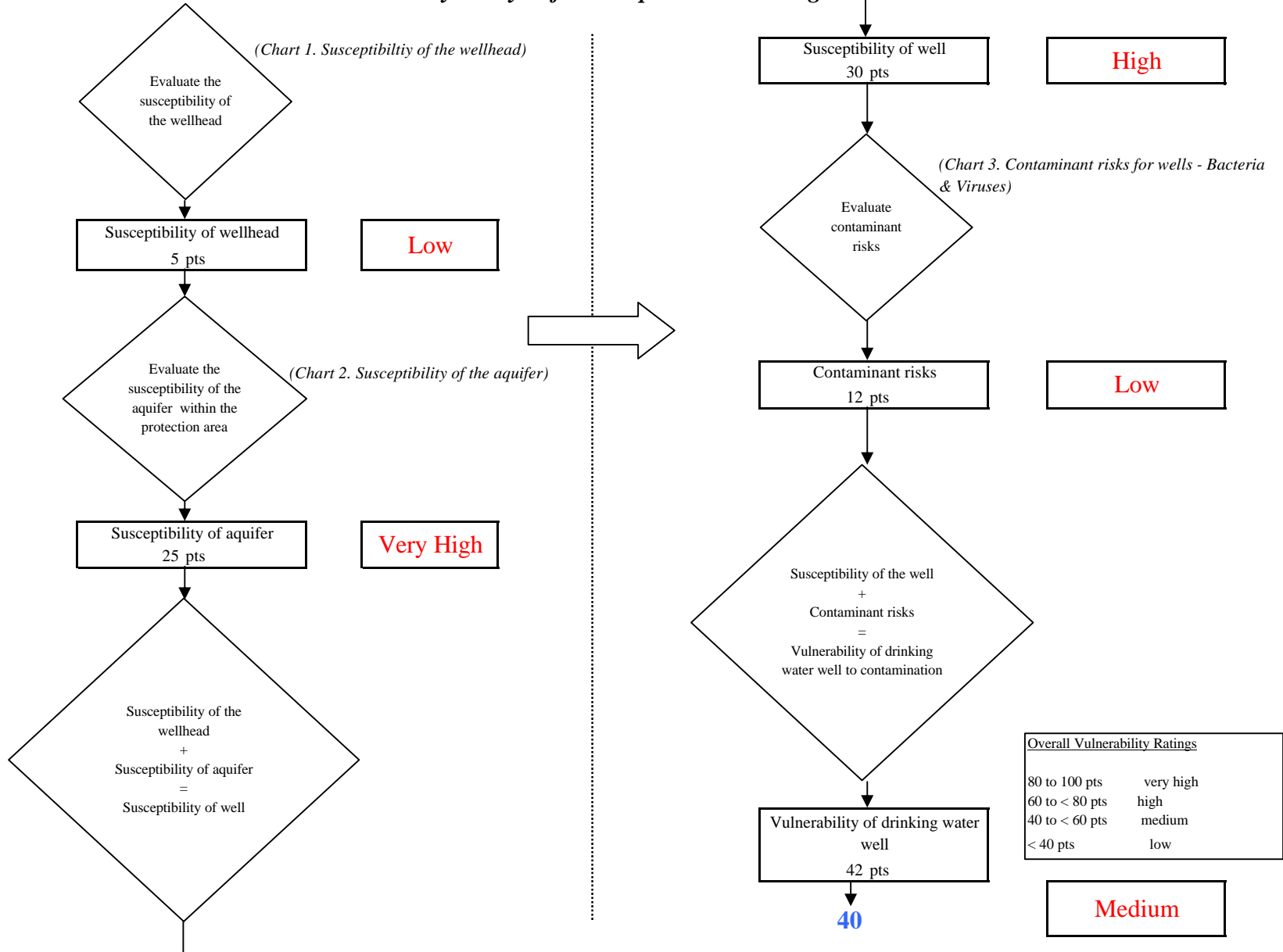
Chart 4. Vulnerability Analysis for Sheep Mountain Lodge - Bacteria & Viruses
