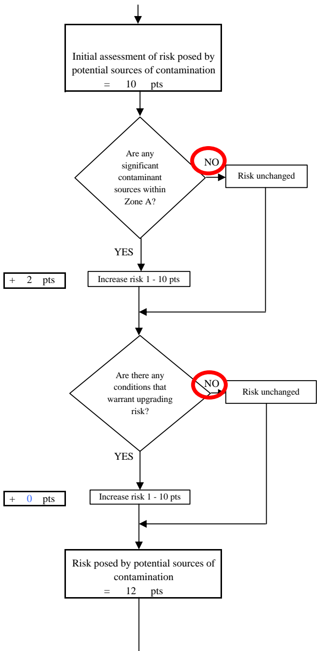
Chart 3. Contaminant Risks for Sheep Mountain Lodge - Bacteria & Viruses
