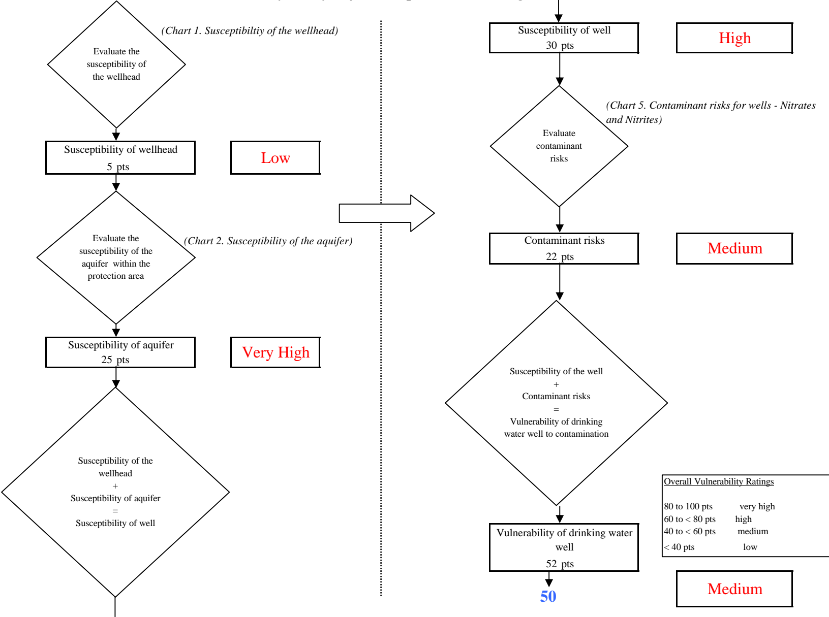
Chart 6. Vulnerability Analysis for Sheep Mountain Lodge - Nitrates and Nitrites
