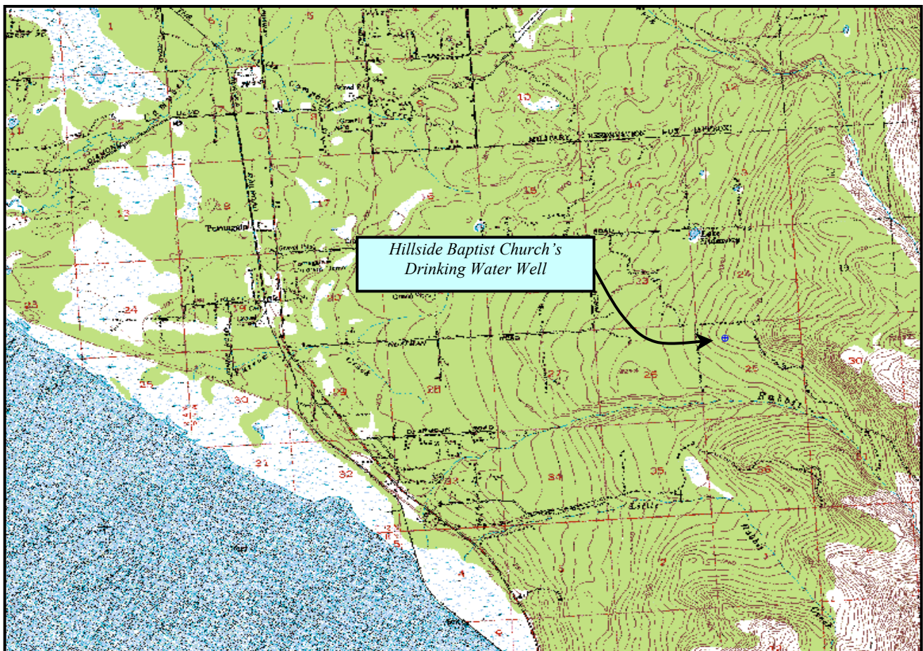
Figure 3. Map showing the location of the drinking water source for Hillside Baptist Church [Base: USGS Anchorage A8].
