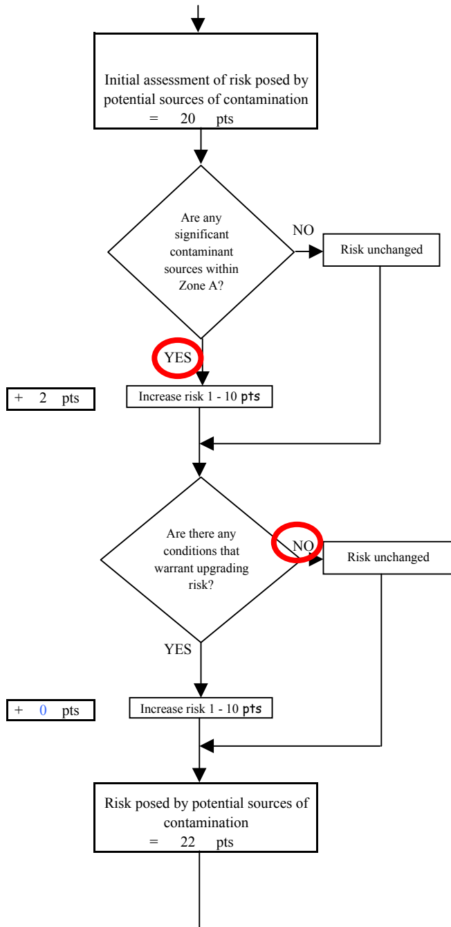
Chart 3. Contaminant risks for Hillside Baptist Church - Bacteria & Viruses
