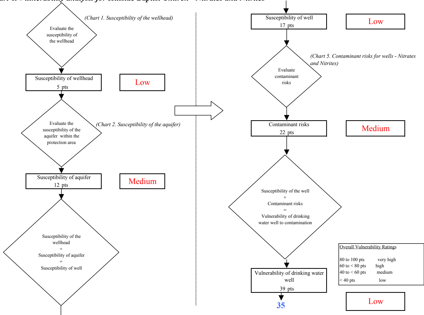
Chart 6. Vulnerability analysis for Hillside Baptist Church - Nitrates and Nitrites
