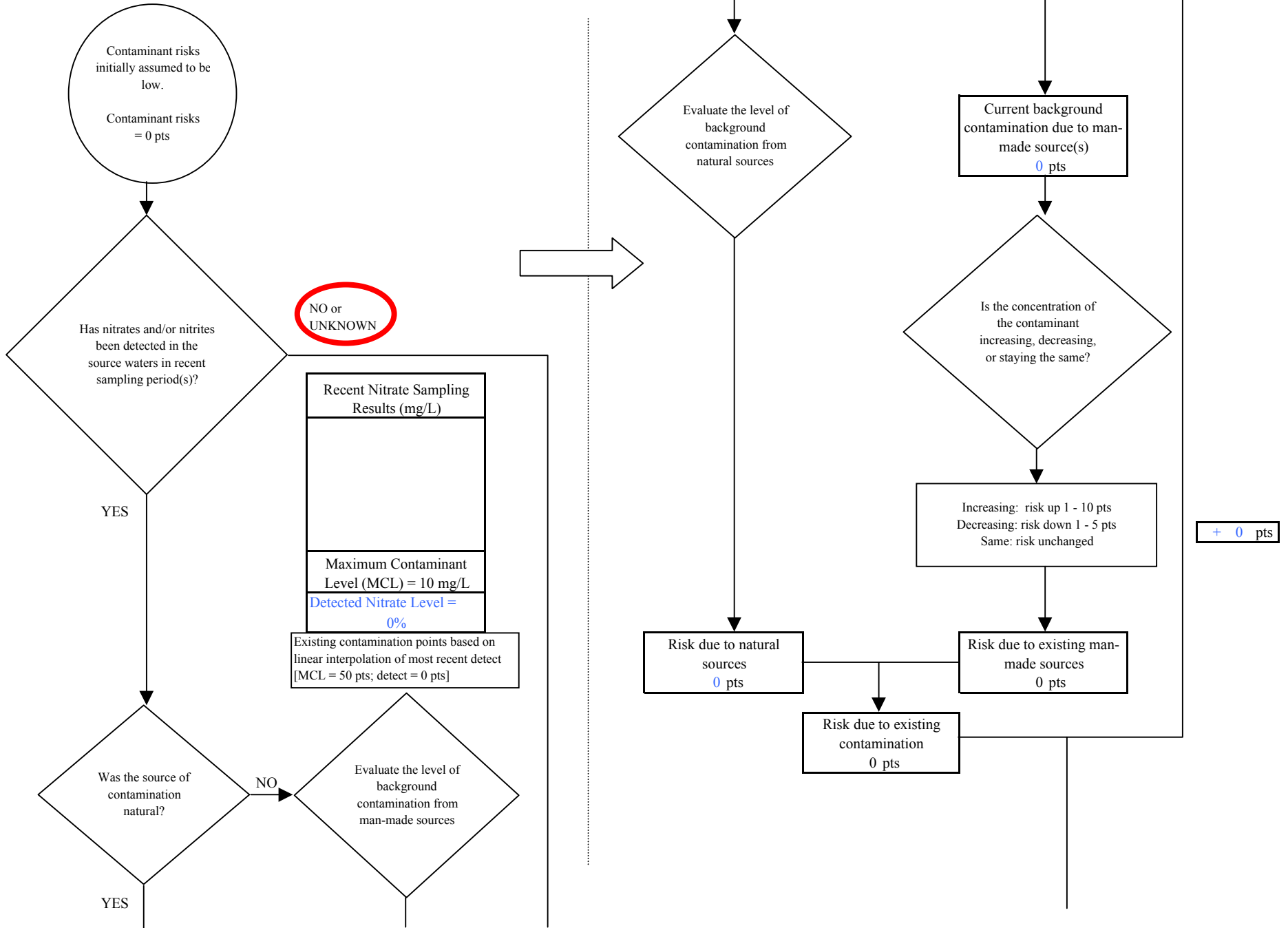
Chart 5. Contaminant risks for Hillside Baptist Church - Nitrates and Nitrites
