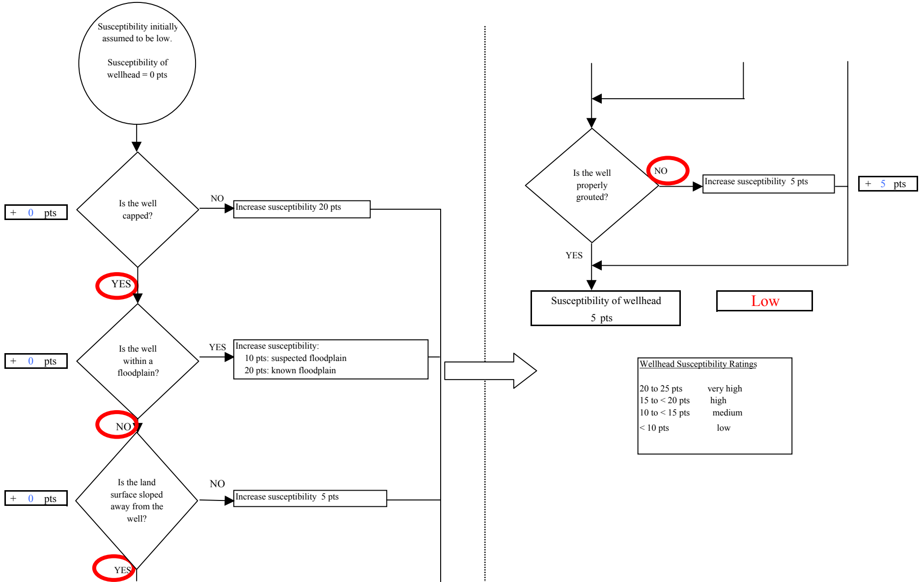
Chart 1. Susceptibility of the wellhead - Hillside Baptist Church
