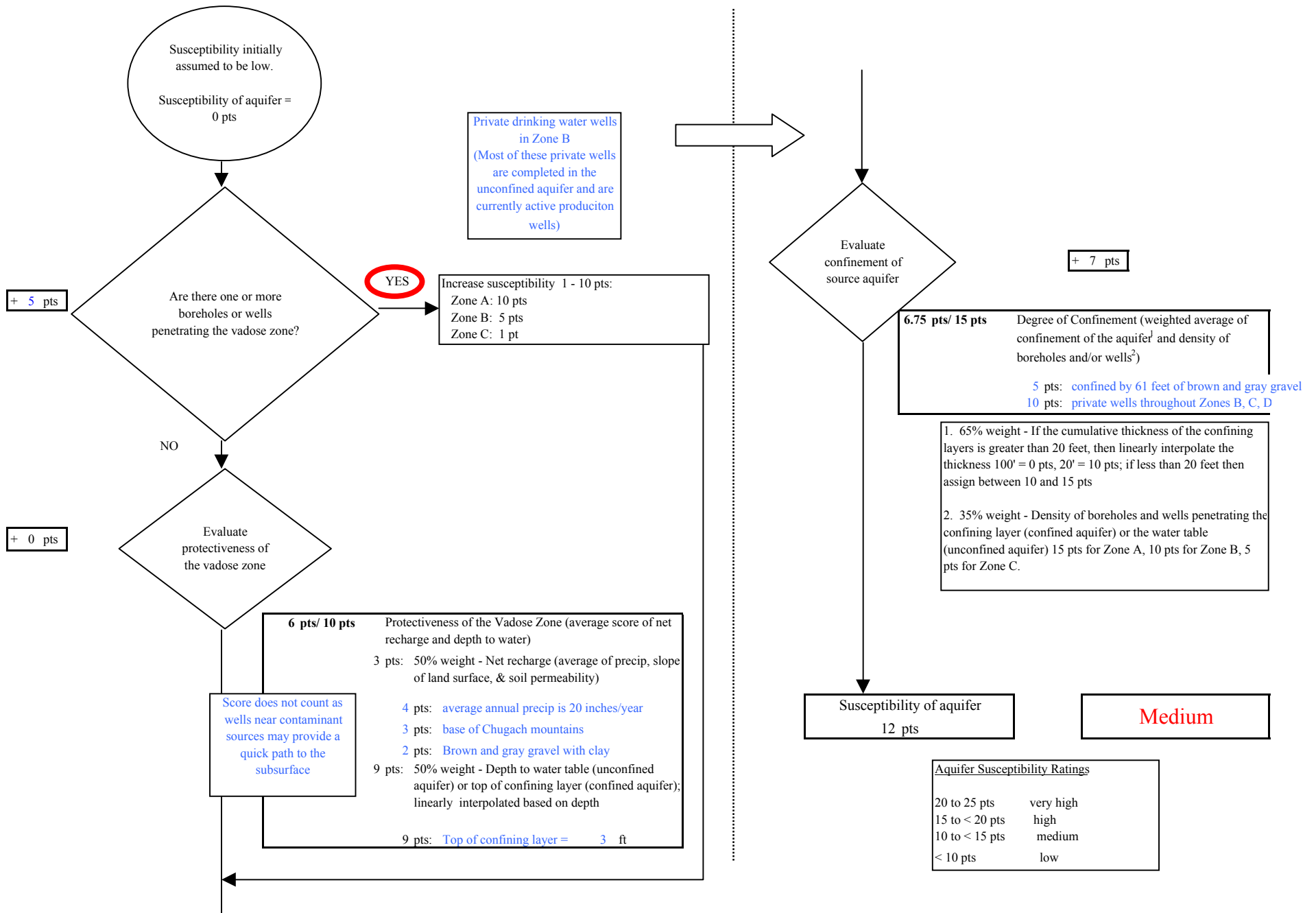
Chart 2. Susceptibility of the aquifer - Hillside Baptist Church
