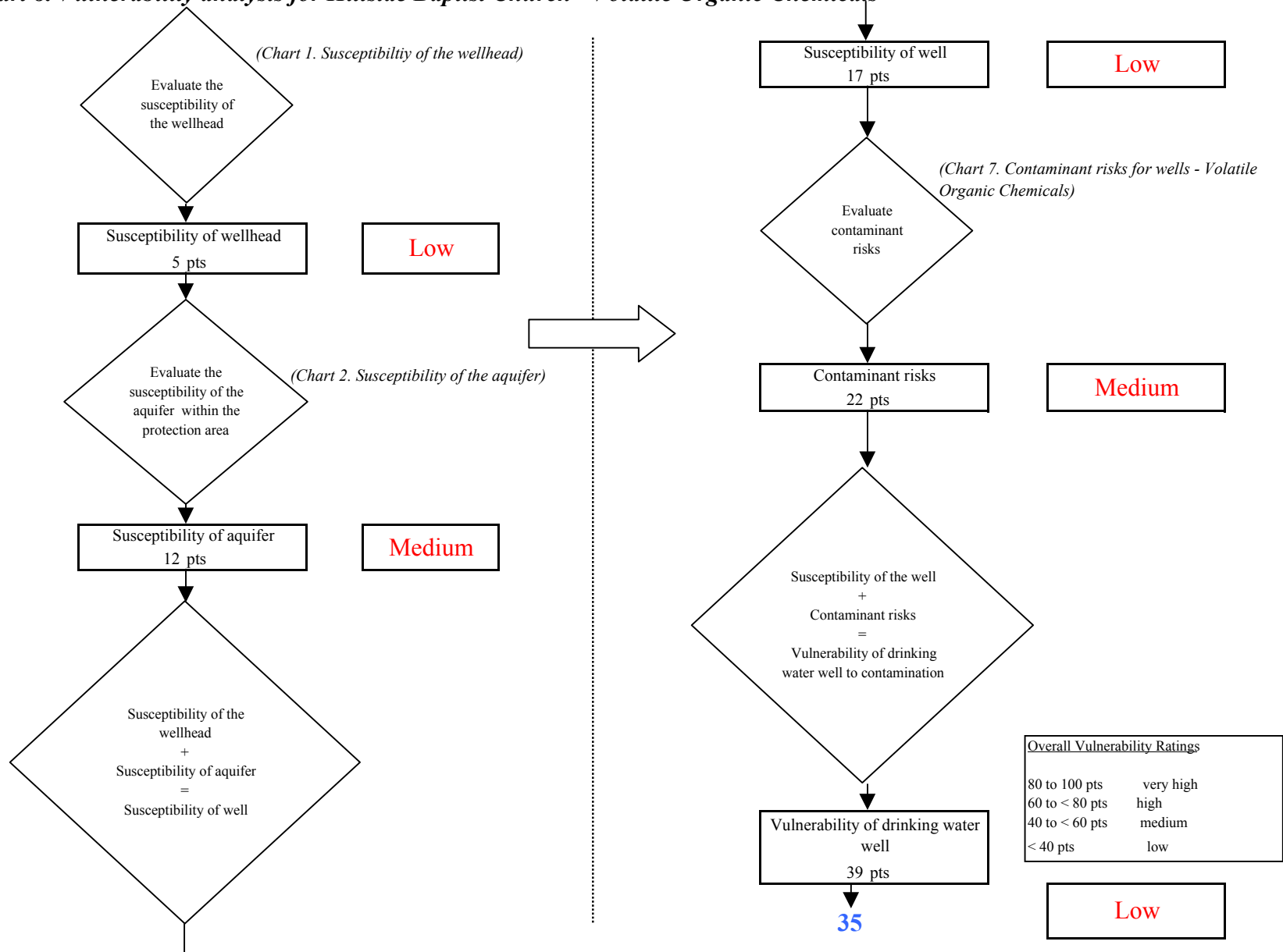
Chart 8. Vulnerability analysis for Hillside Baptist Church - Volatile Organic Chemicals
