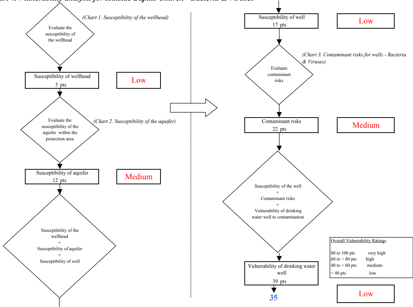
Chart 4. Vulnerability analysis for Hillside Baptist Church - Bacteria & Viruses
