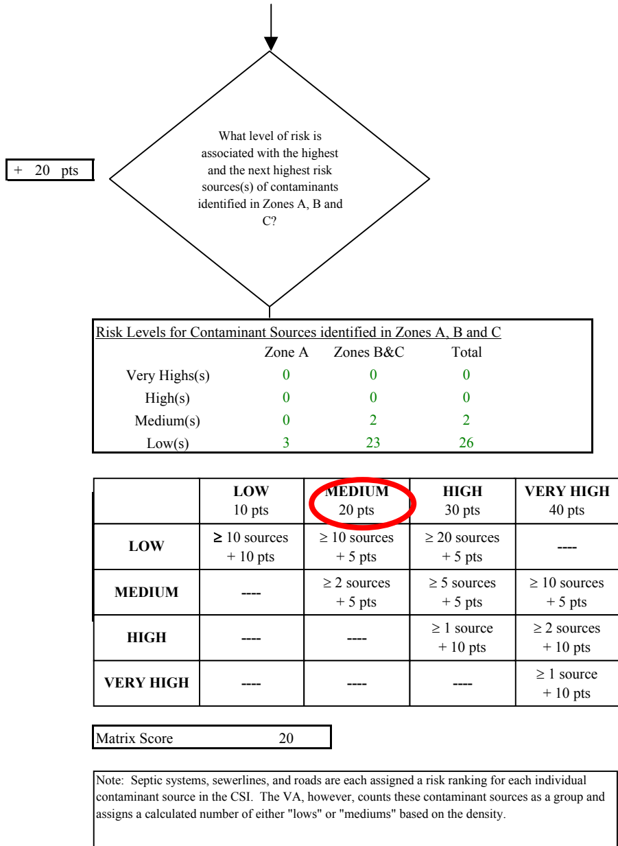
Chart 5. Contaminant risks for Hillside Baptist Church - Nitrates and Nitrites
