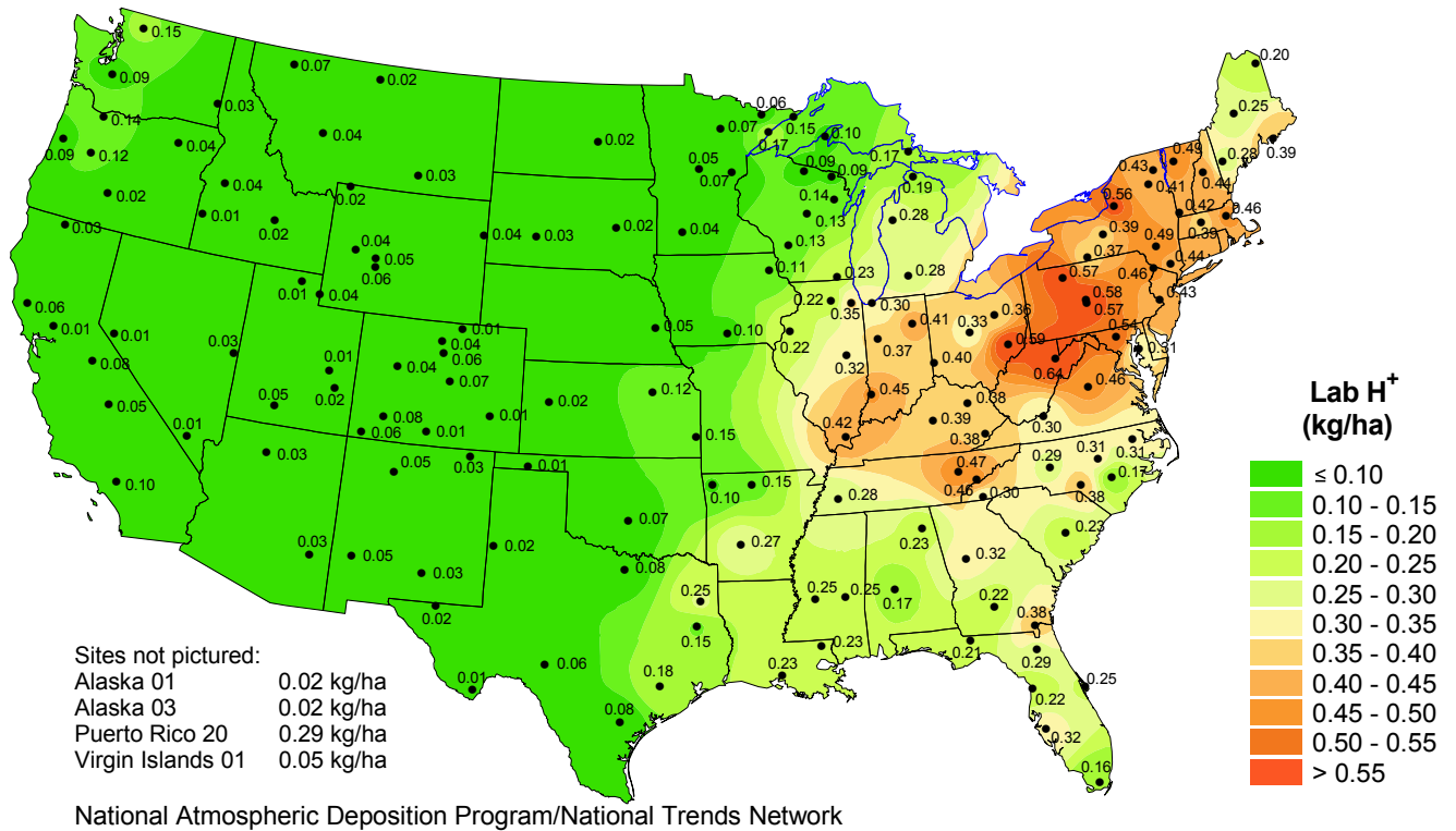
Hydrogen ion concentration as pH (top) and estimated deposition (bottom) from measurements made at the Central Analytical Laboratory, 1998.
