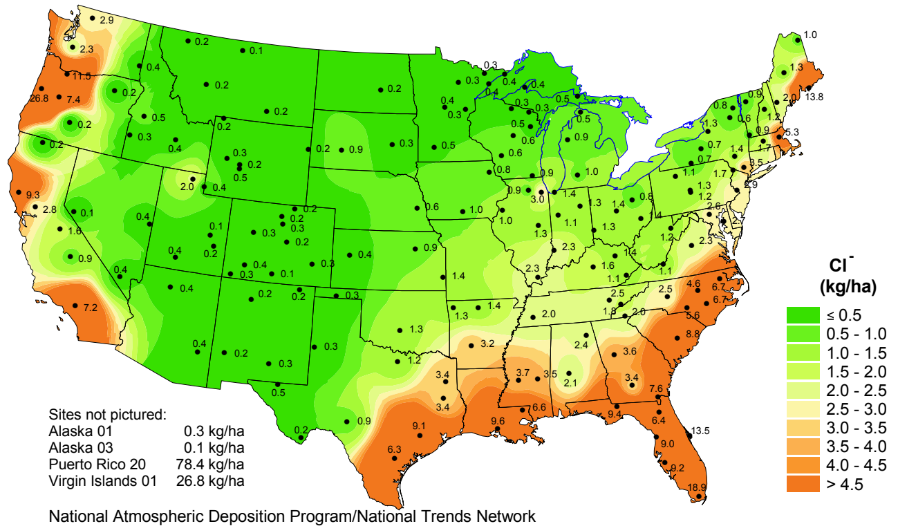
Chloride ion concentration (top) and estimated deposition (bottom), 1998.
