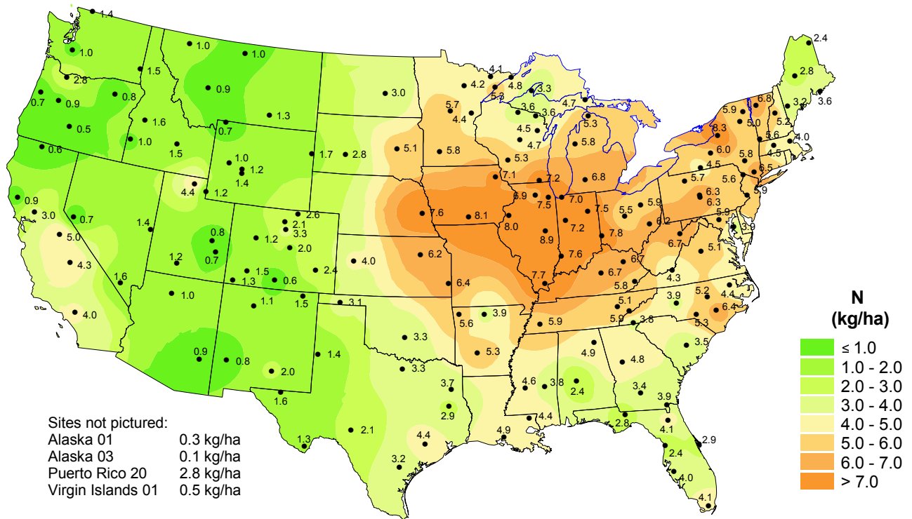
Estimated inorganic nitrogen deposition from nitrate and ammonium, 1998.
