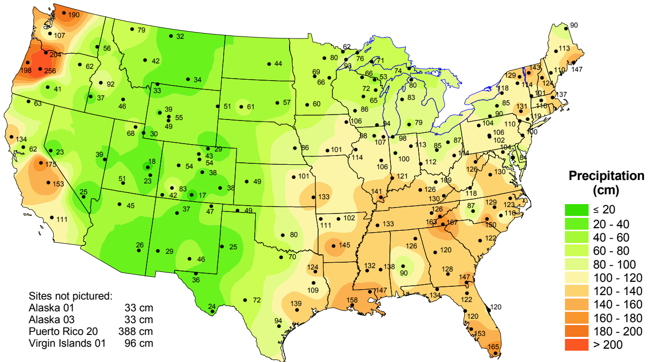
Hydrogen ion concentration as pH from measurements made in field laboratories (top) and total precipitation (bottom), 1998.
