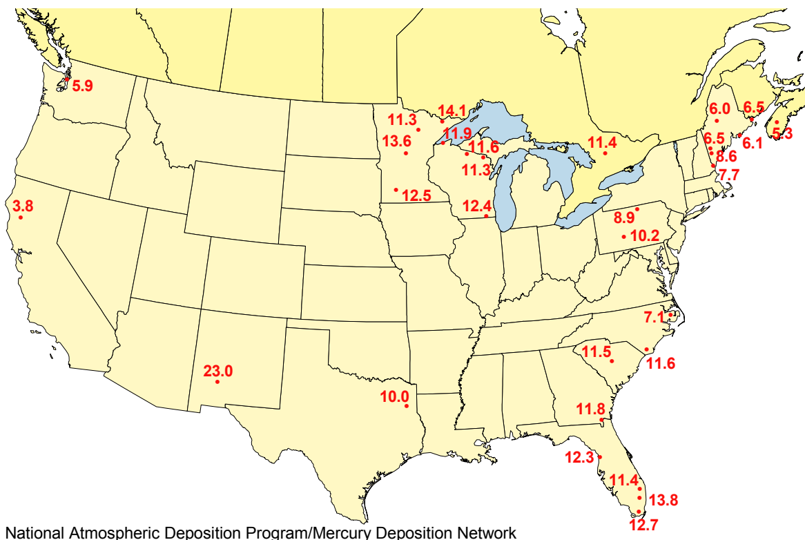
Mercury concentration in ng/L, 1998
