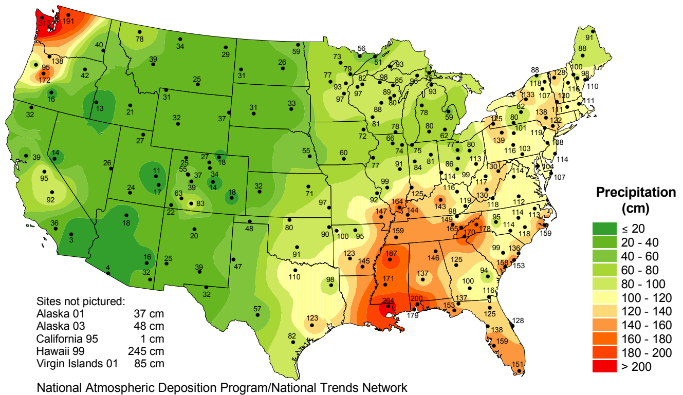
Total precipitation, 2002.
