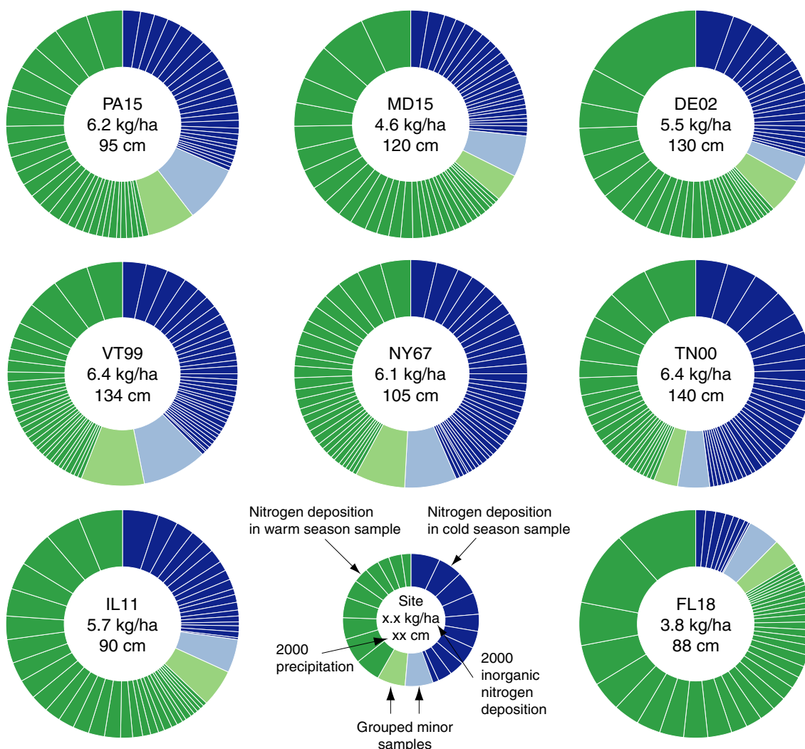
Contributions of individual samples to inorganic nitrogen wet deposition at AIRMoN sites, 2000. Minor samples contributing less than 0.5 percent are grouped.
