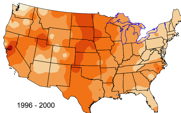
Percent of Inorganic Nitrogen Wet Deposition from Ammonium
