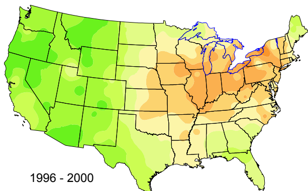
Inorganic Nitrogen Wet Deposition from Nitrate and Ammonium (kg/ha)
