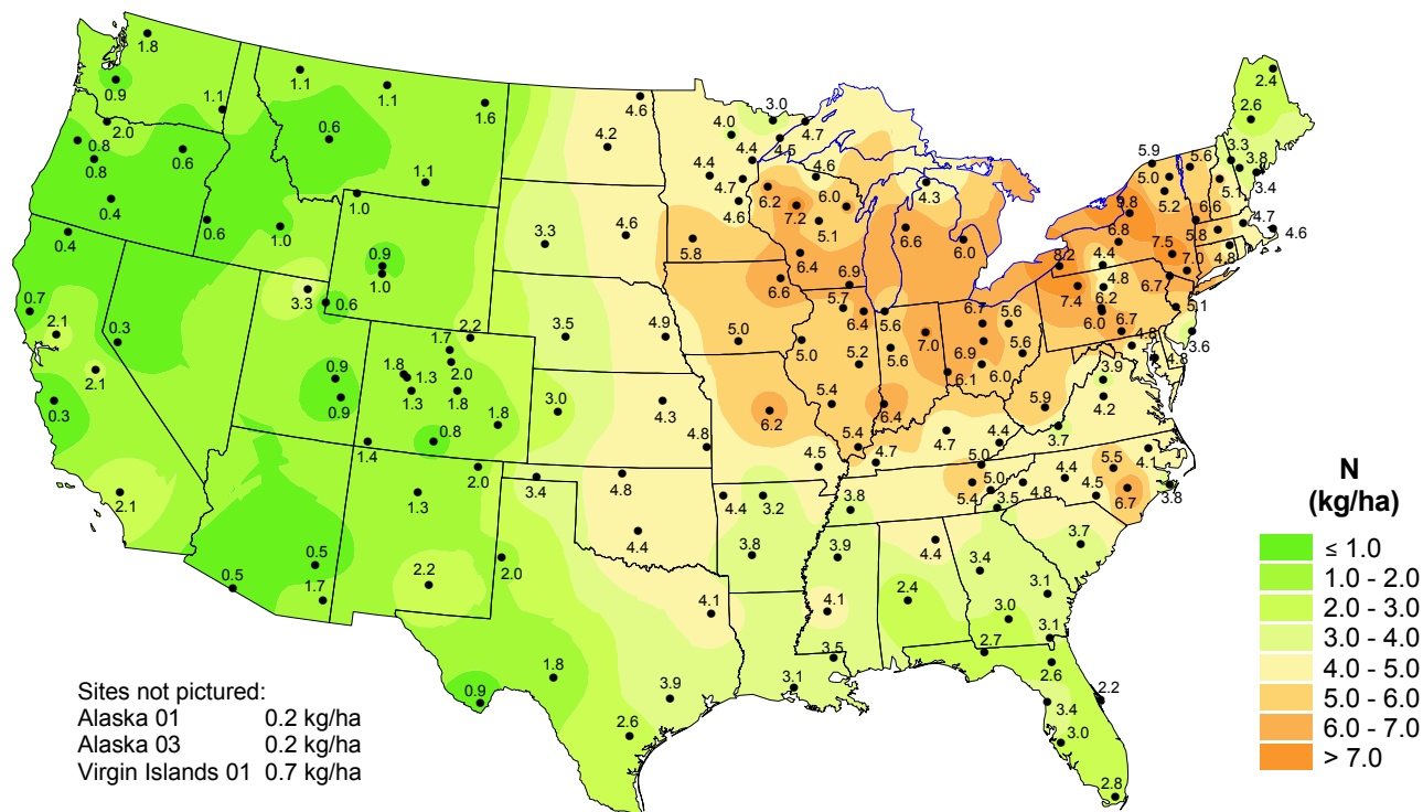
Inorganic nitrogen wet deposition from nitrate and ammonium, 2000
